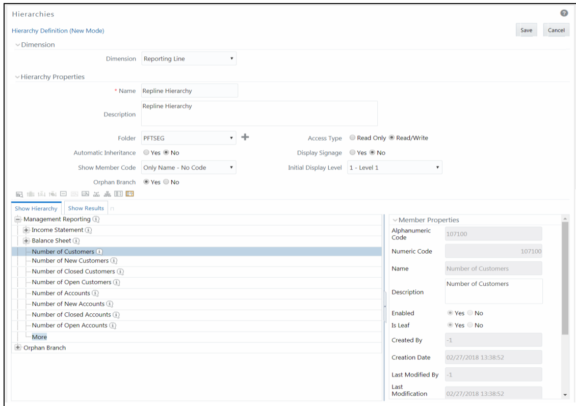
Figure 36: Hierarchies window
