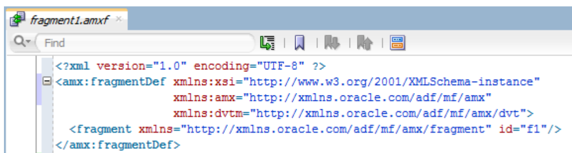
Figure 13-43 Fragment File
