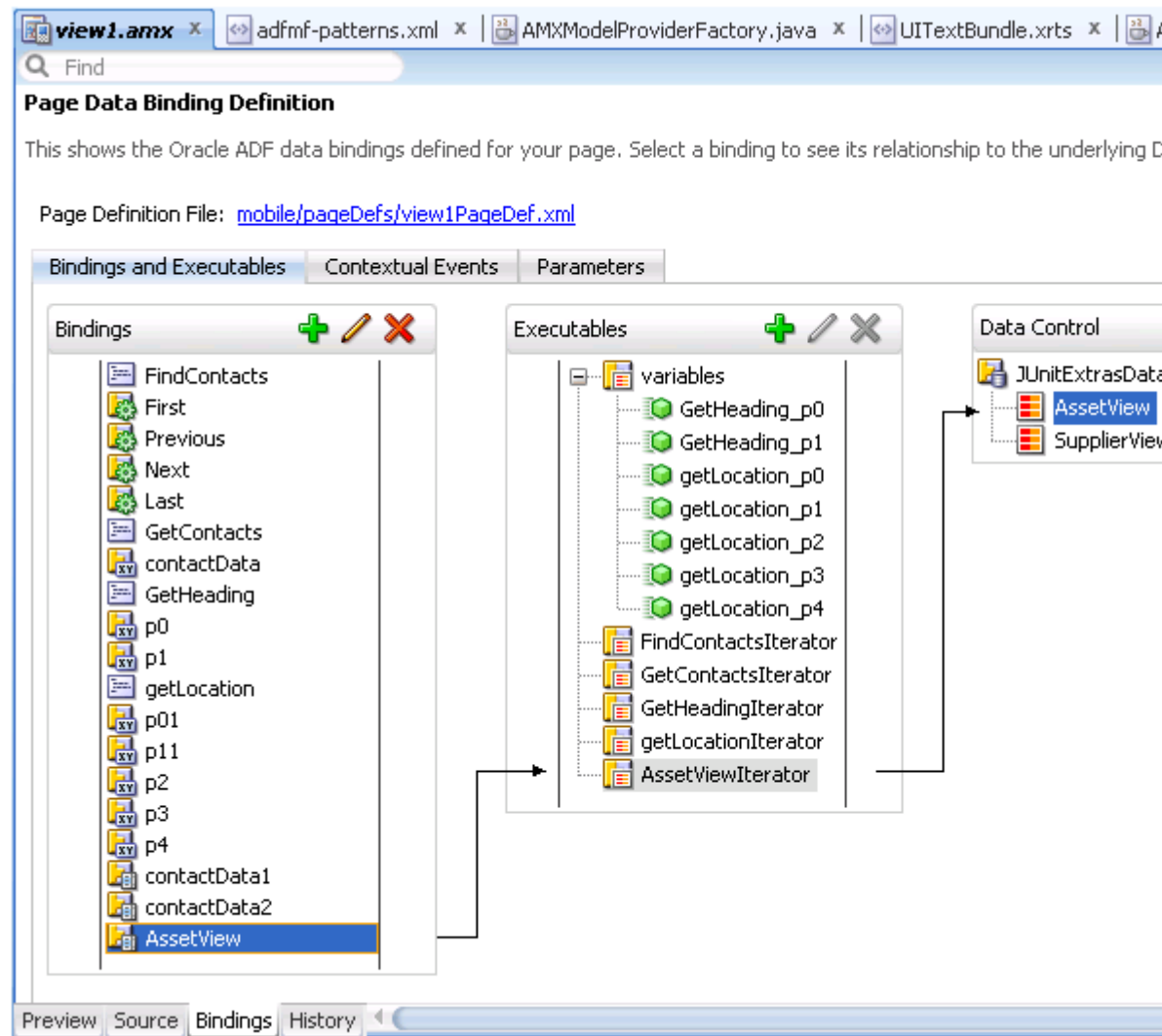
Figure 13-85 Bindings Tab
