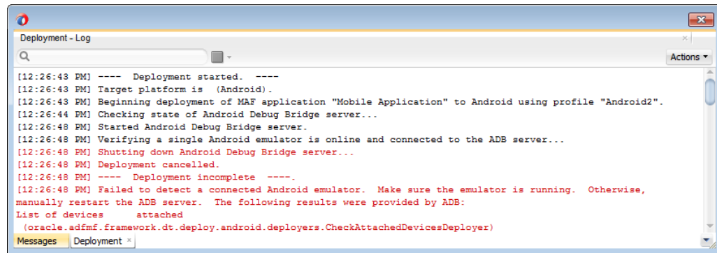
Figure 25-10 Deployment Terminated
