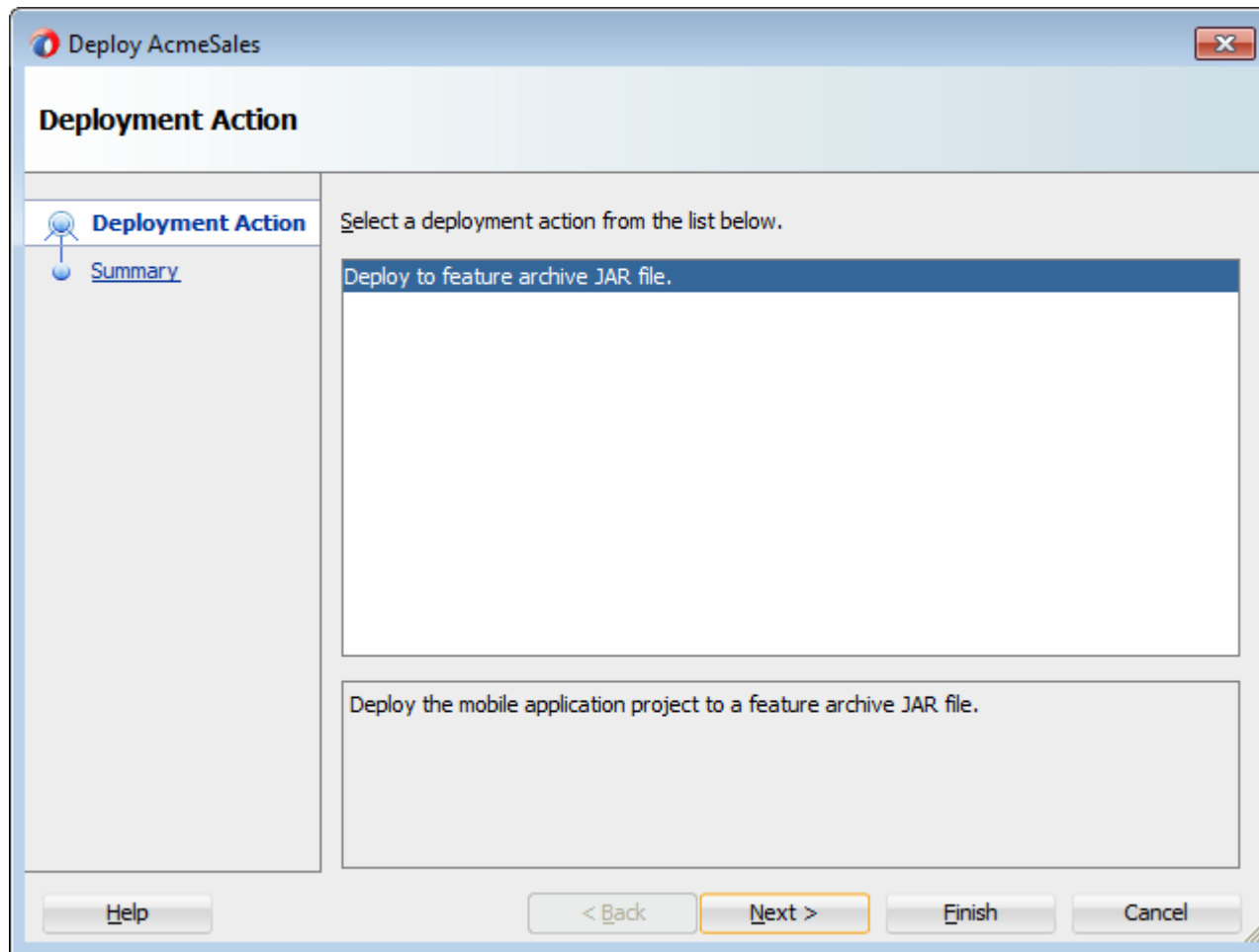
Figure 25-24 Deployment Actions
