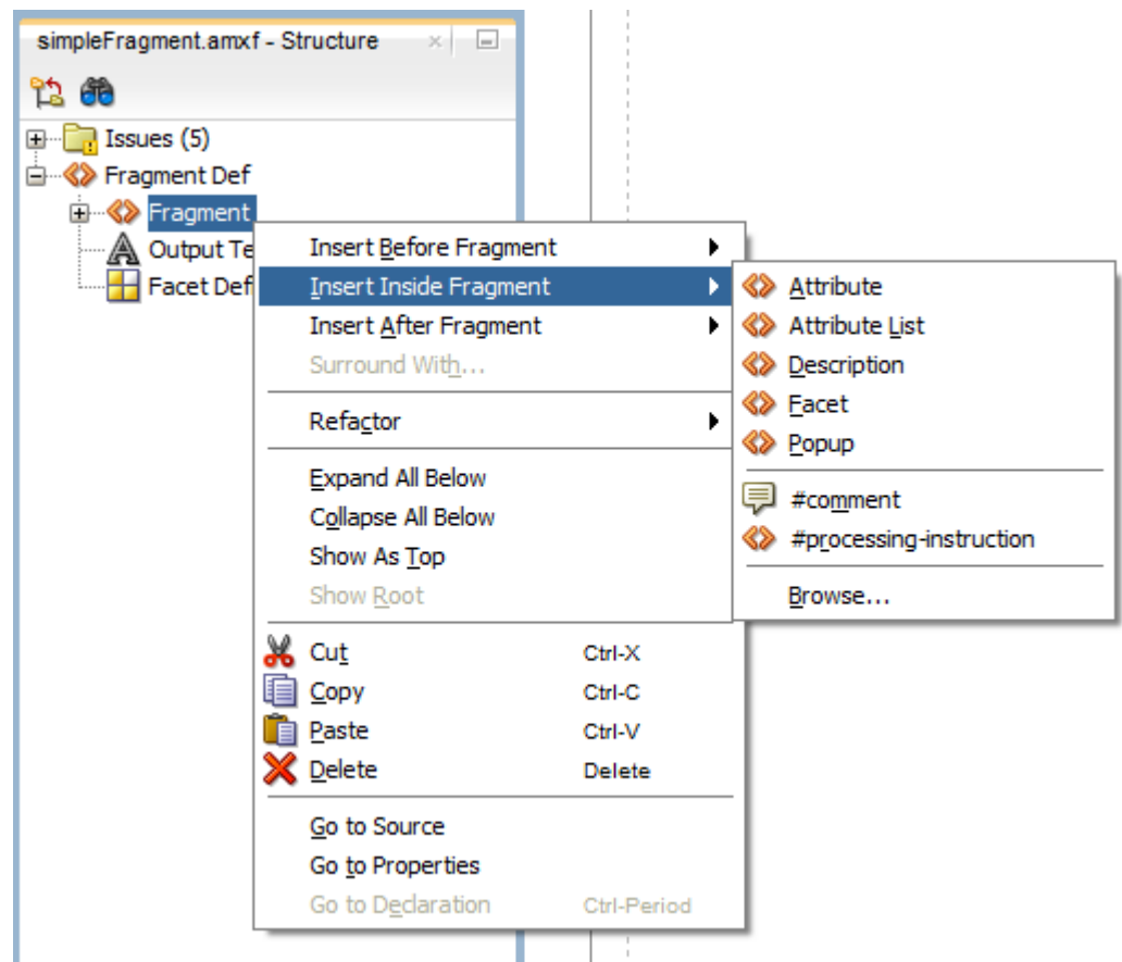
Figure 13-44 Populating Fragment
