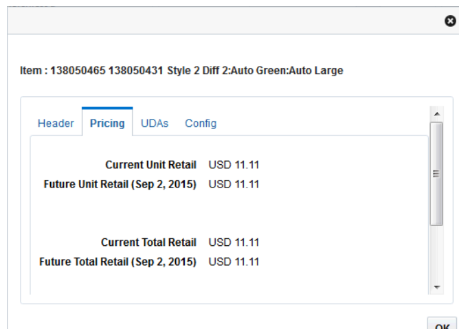
Figure 3–2 Item Window
