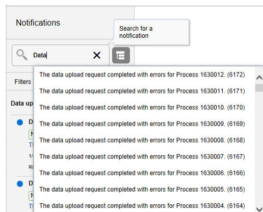
Figure 7–3 Search Bar
