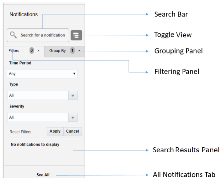
Figure 7–2 Notifications Sidebar
