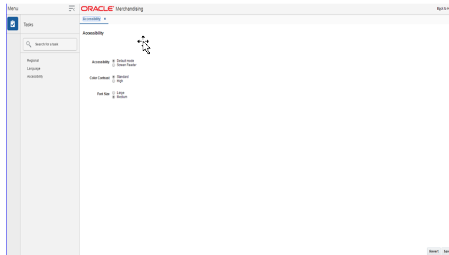
Figure 4–2 Accessibility Tab
