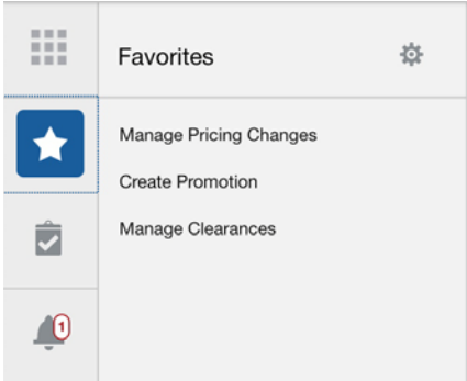
Figure 3–3 Favorites Area
