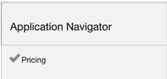
Figure 3–2 Application Navigator
