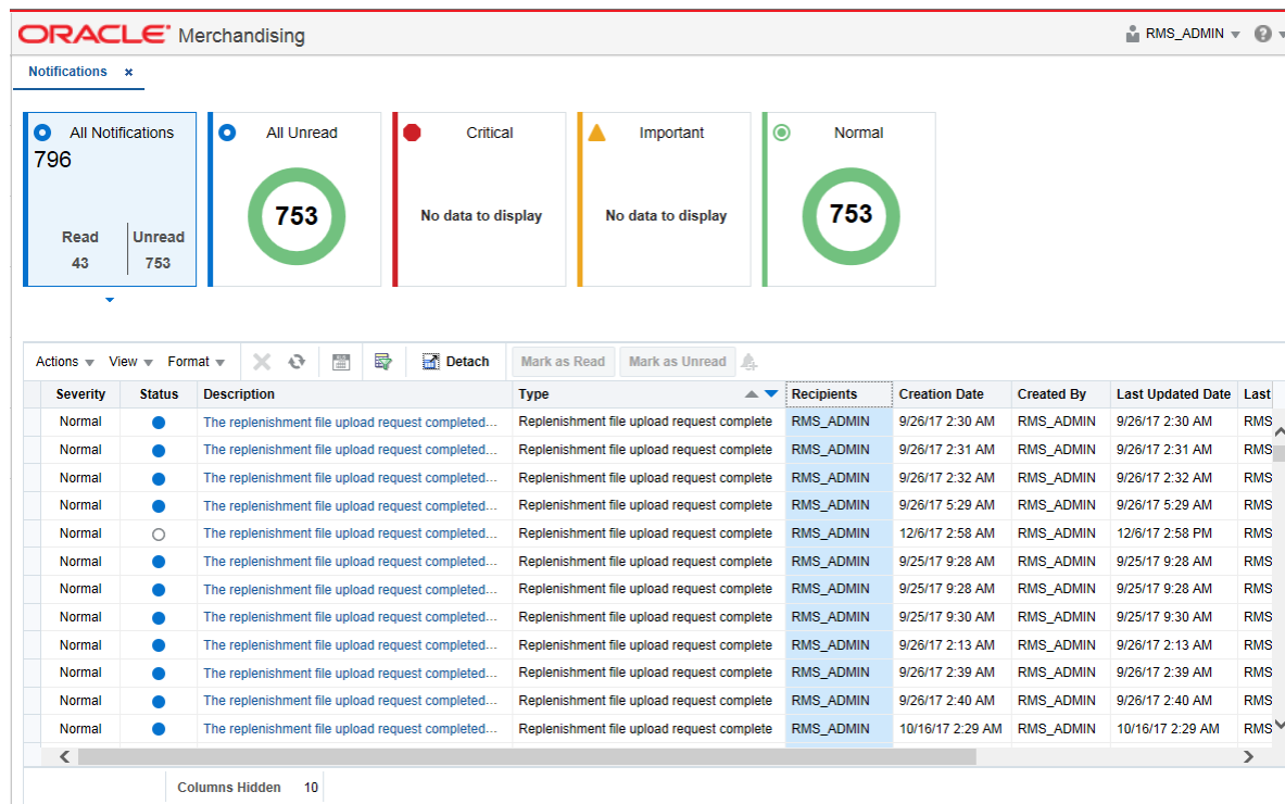
Figure 7–9 All Notifications
