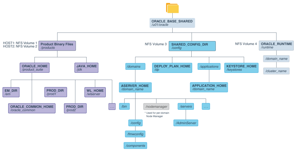
Figure 8-1 Recommended Shared Storage Directory Structure for an Enterprise Deployment
