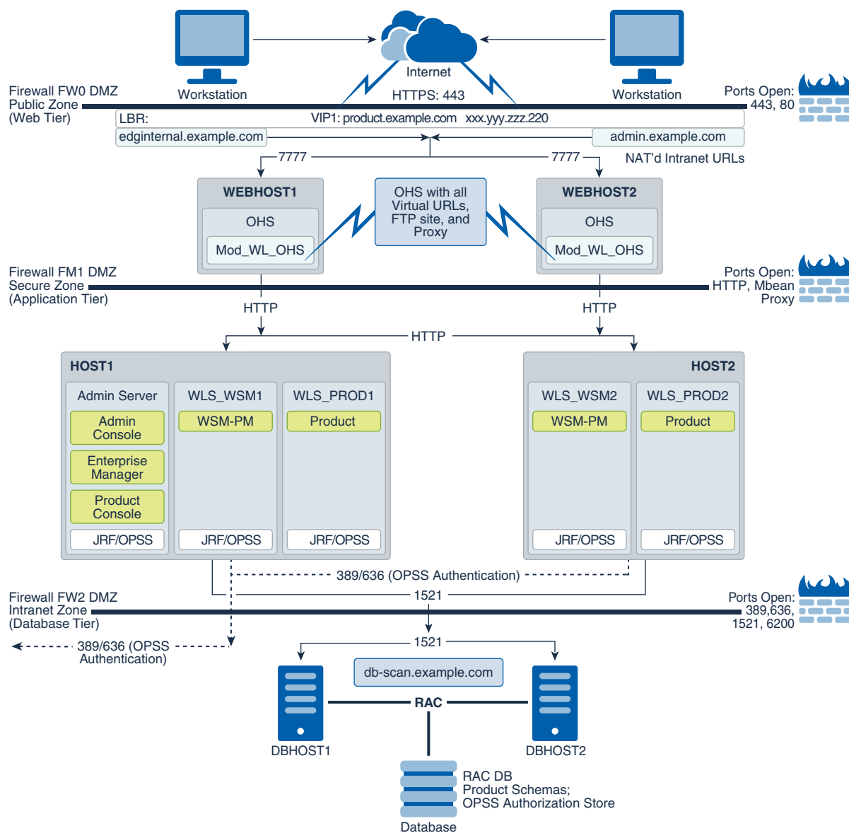
Figure 2-1 Typical Enterprise Deployment Topology Diagram
