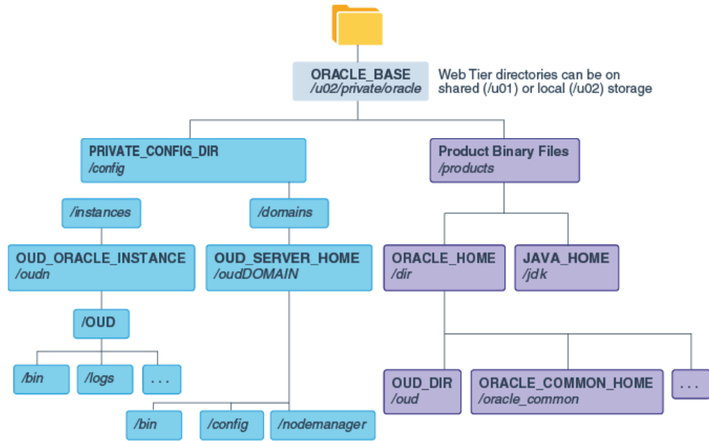
Figure 8-3 Recommended Local Storage Directory Structure for a Directory Tier Host Computer in an Enterprise Deployment
