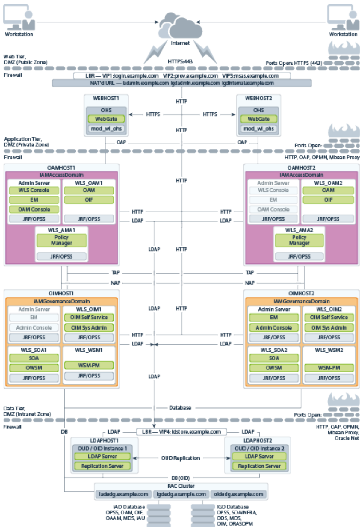
Figure 3-1 Oracle Identity and Access Management Topology
