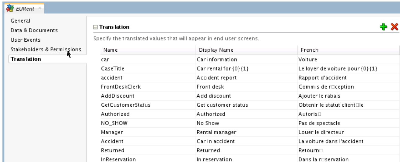
Figure 33-6 Translation Editor
