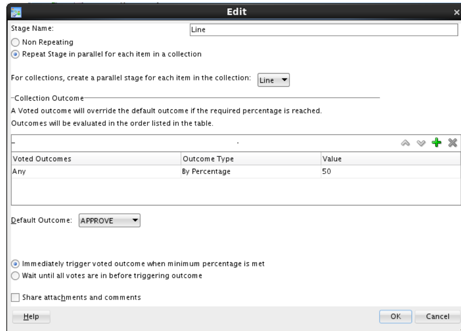
Figure 32-17 Edit Stage Dialog: Repeat Stage
