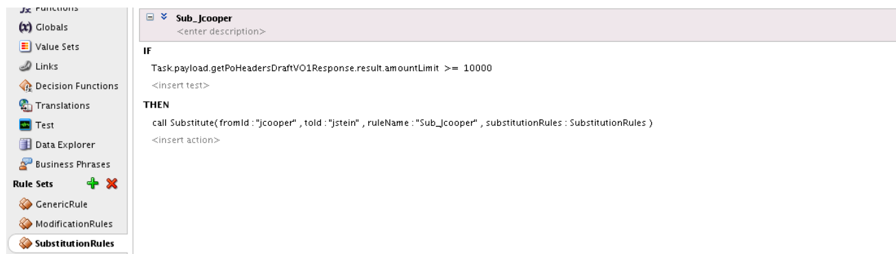
Figure 32-30 Sample Approver-Substitution Action
