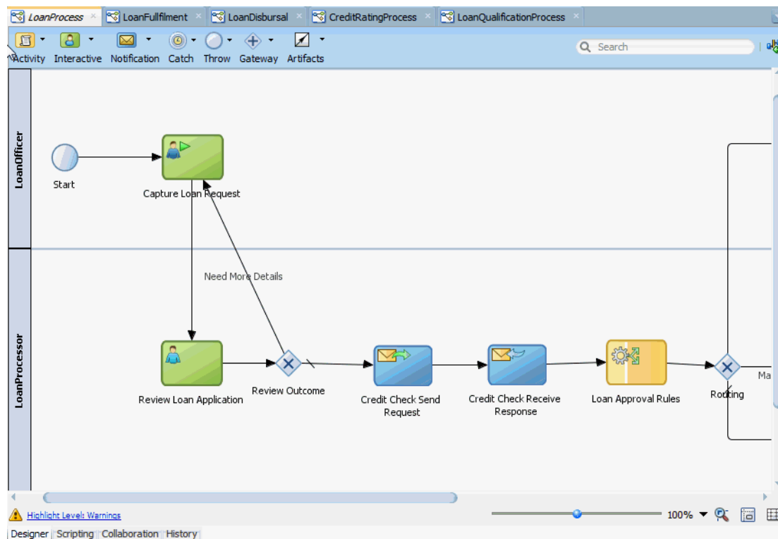
Figure 1-4 Process Editor
