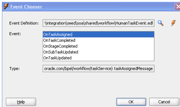
Figure 29-65 Event Callbacks
