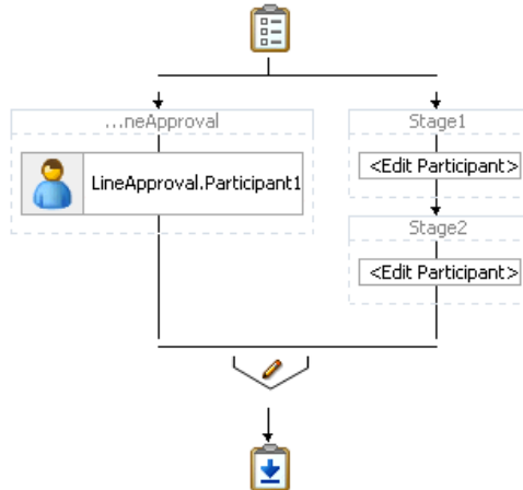
Figure 29-19 Sequential Stage
