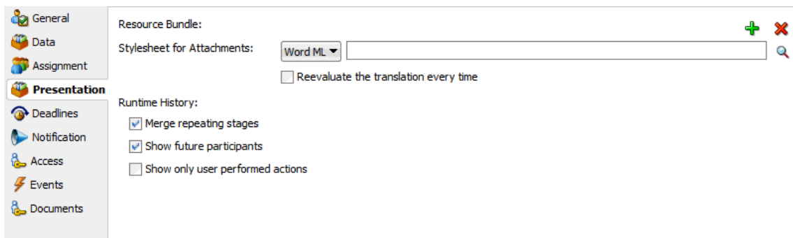
Figure 29-51 Presentation Section
