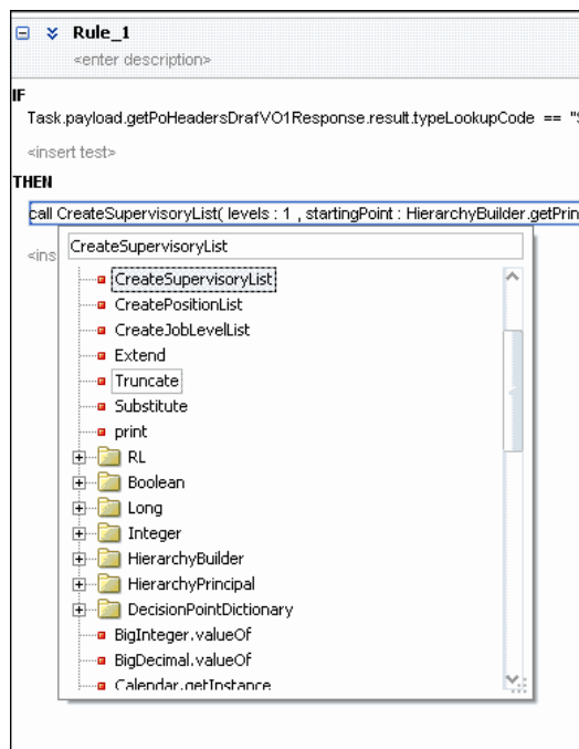
Figure 32-31 Rule Functions
