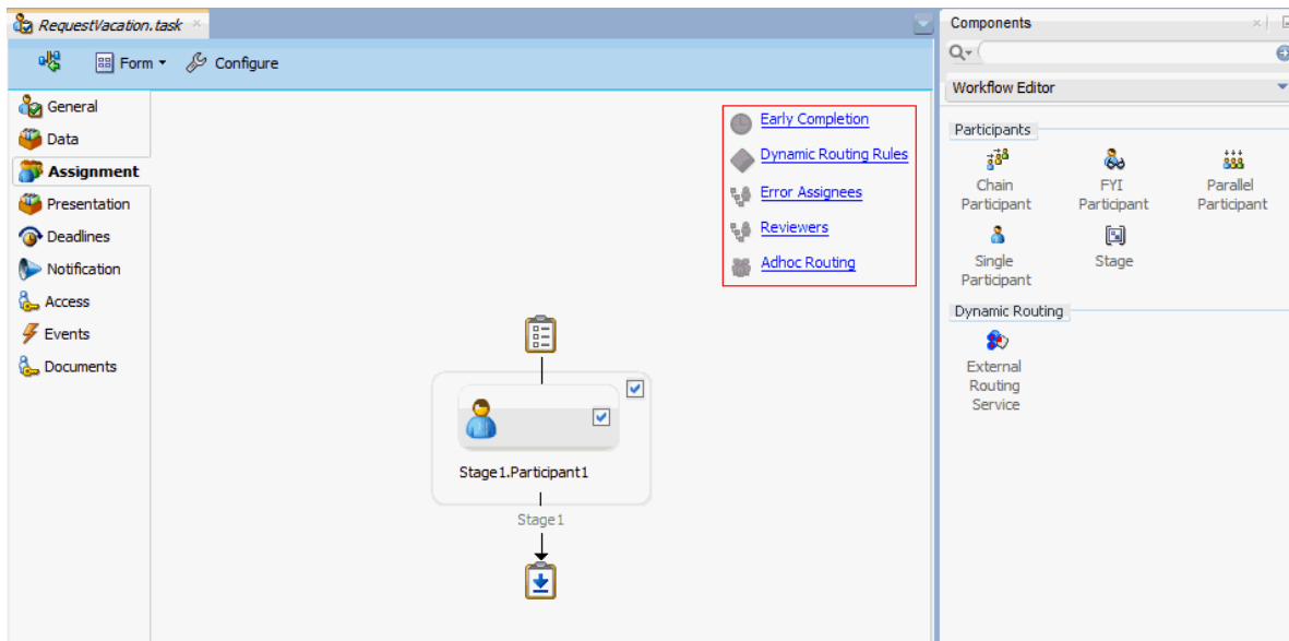
Figure 29-16 Human Task Editor — Assignment Section
