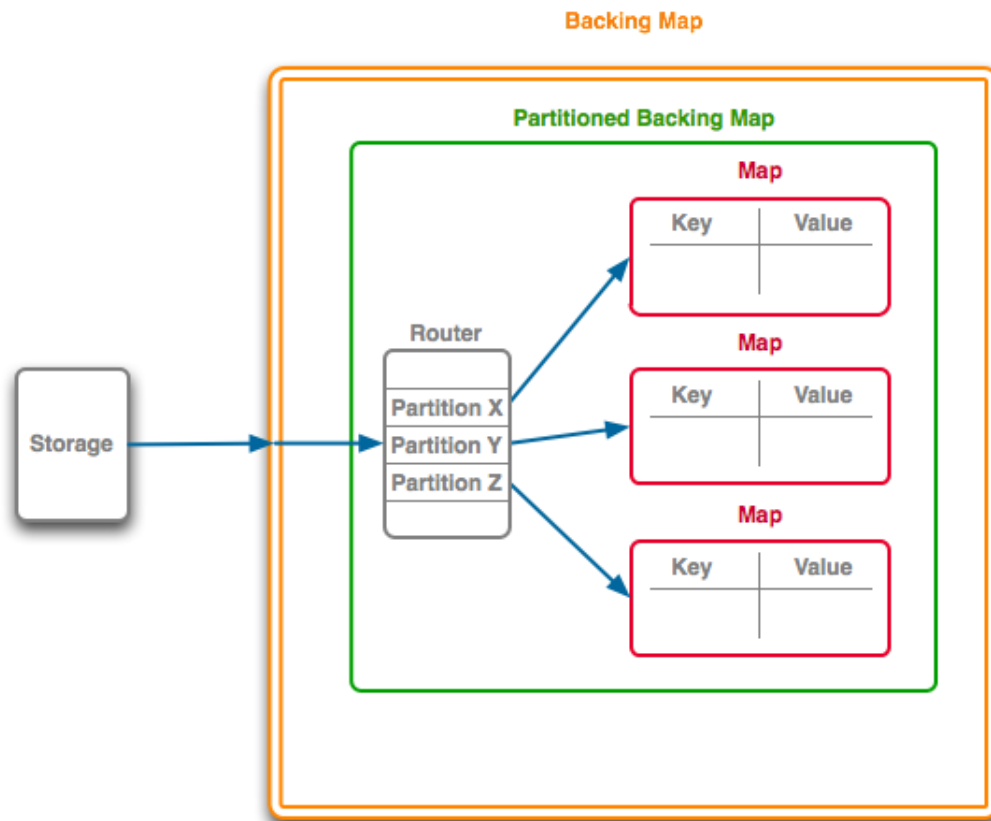
Figure 13-3 Partitioned Backing Map Implementation
