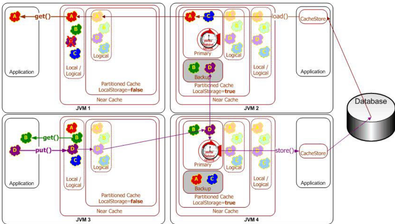
Figure 14-3 Write-Behind Caching
