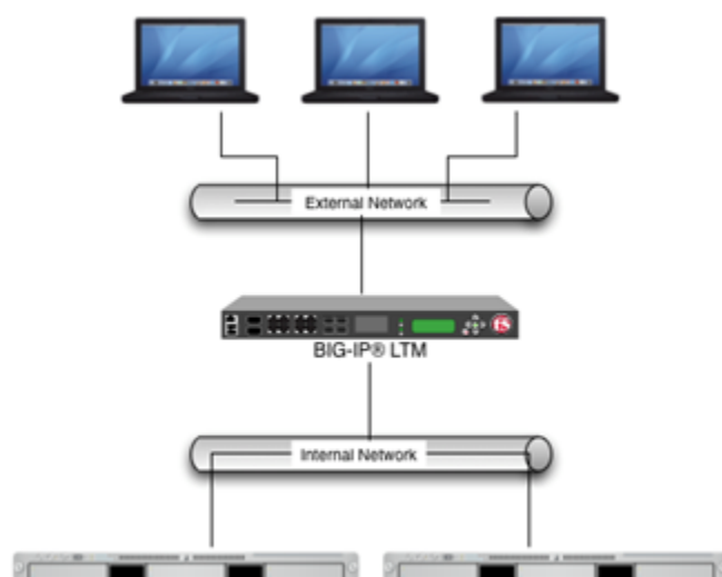
Figure B-1 Conceptual View of F5 BIG-IP LTM
