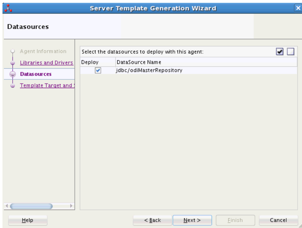
Figure 3-3 Server Template Generation Wizard - Datasources Tab
