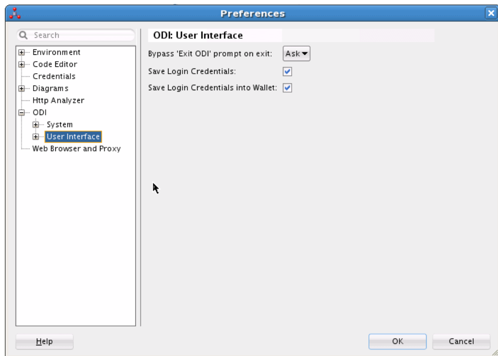
Figure 11-3 Preferences Dialog Box for Saving Login Credentials
