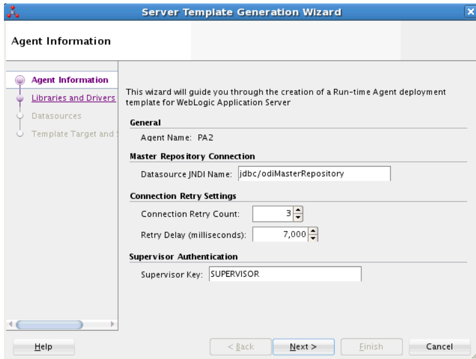
Figure 3-1 Server Template Generation Wizard - Agent Information Tab
