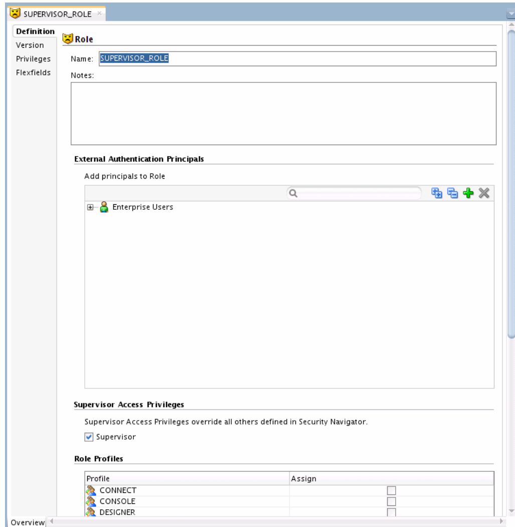
Figure 11-11 Roles Editor
