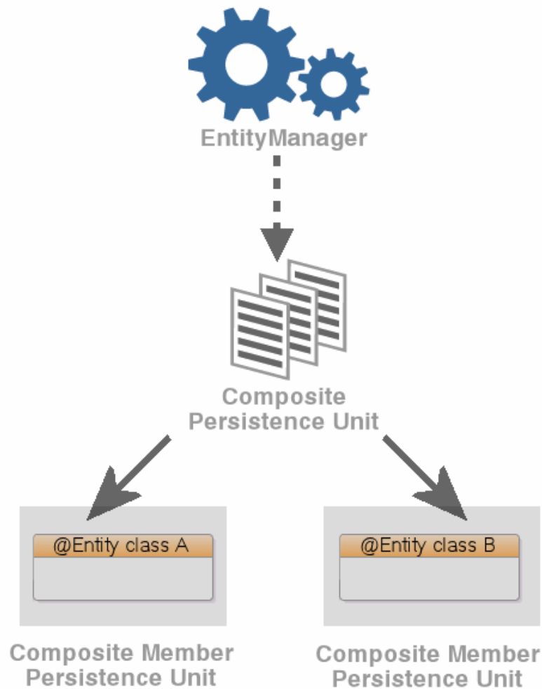
Figure 9-1 A Simple Composite Persistence Unit
