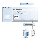
Figure 3-1 Relationship of WebLogic Server, TopLink, and Related Products
