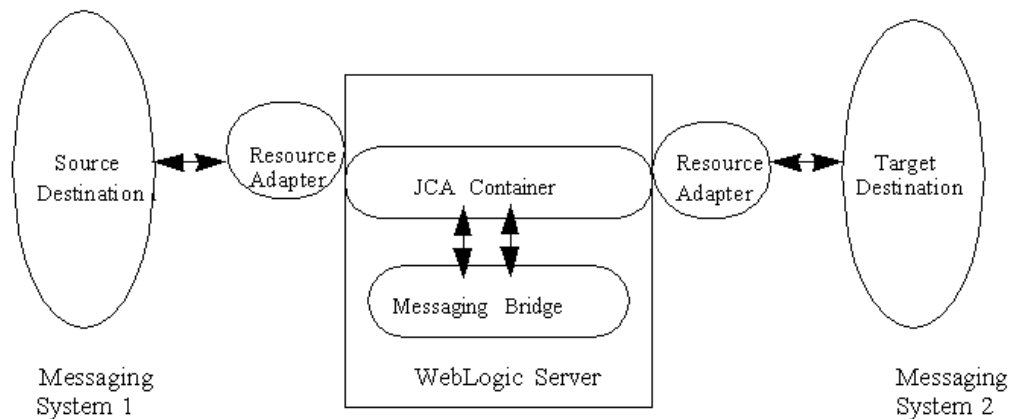
Figure 2-1 WebLogic Messaging Bridge
