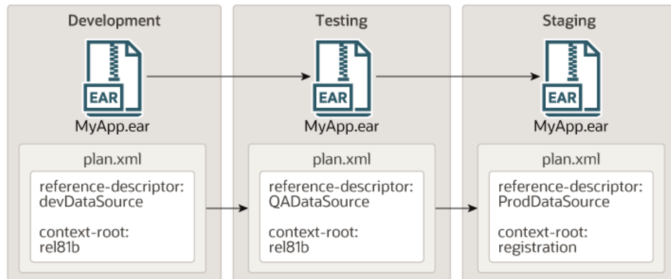
Figure 4-2 Single Deployment Plan Workflow
