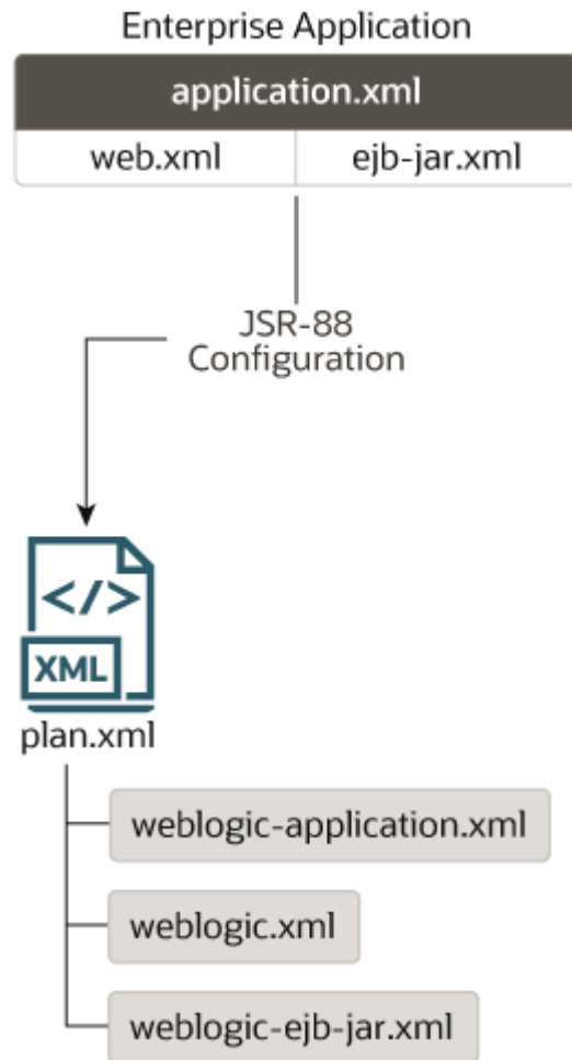
Figure 2-1 Configuring Applications with the Java EE Deployment API
