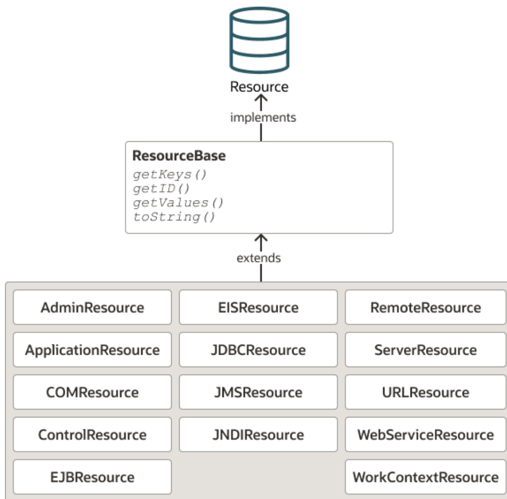
Figure 2-10 Architecture of WebLogic Resources
