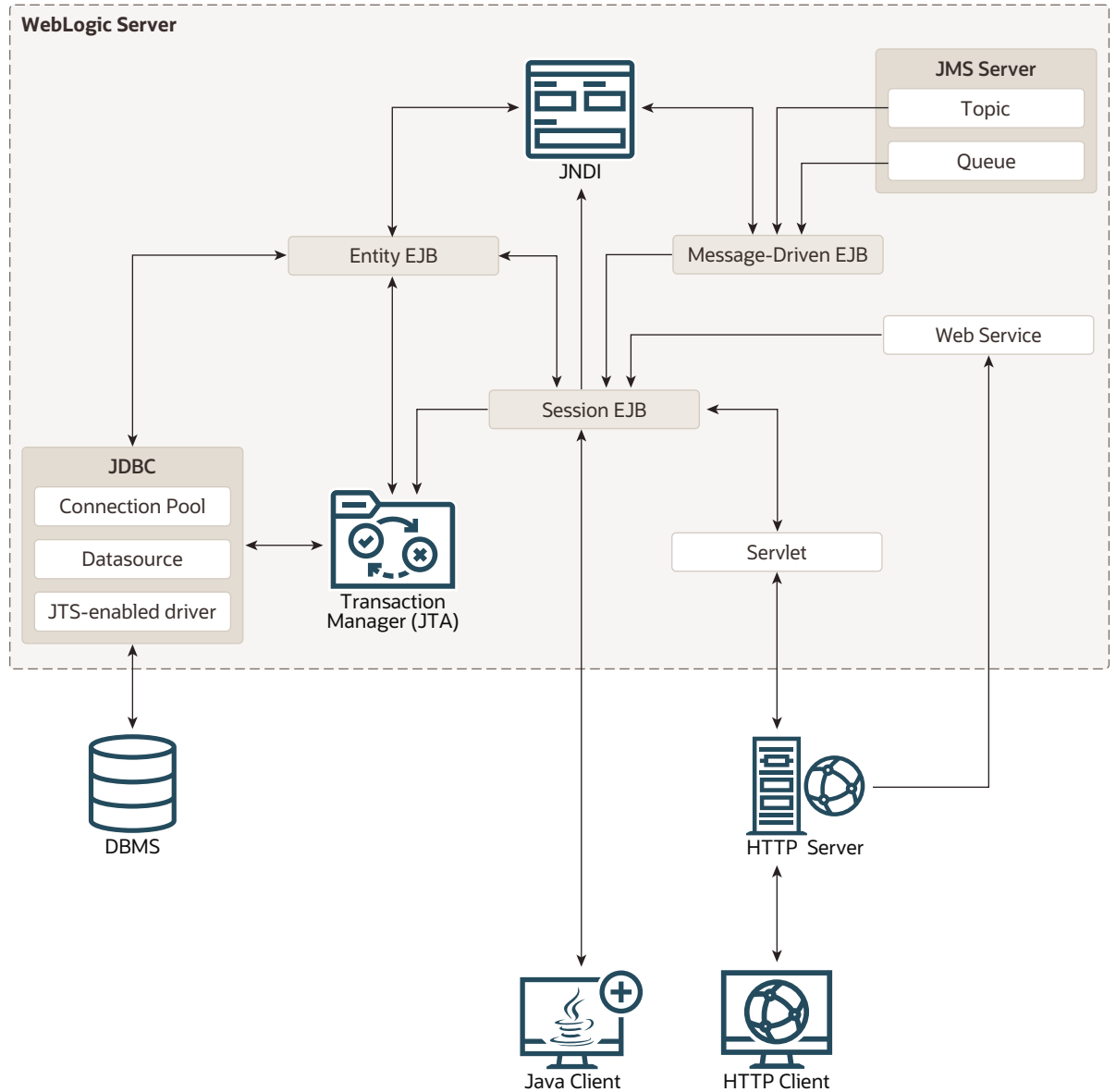
Figure 2-1 EJBs and Other Application Components
