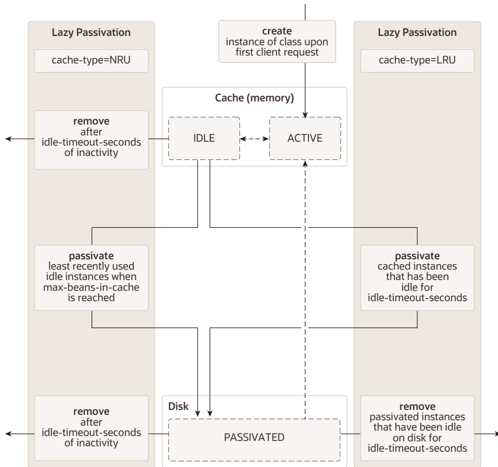
Figure 5-2 Stateful Session EJB Life Cycle
