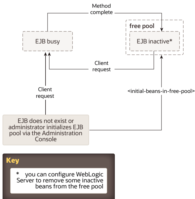
Figure 5-1 WebLogic Server Free Pool Showing Stateless Session EJB Life Cycle
