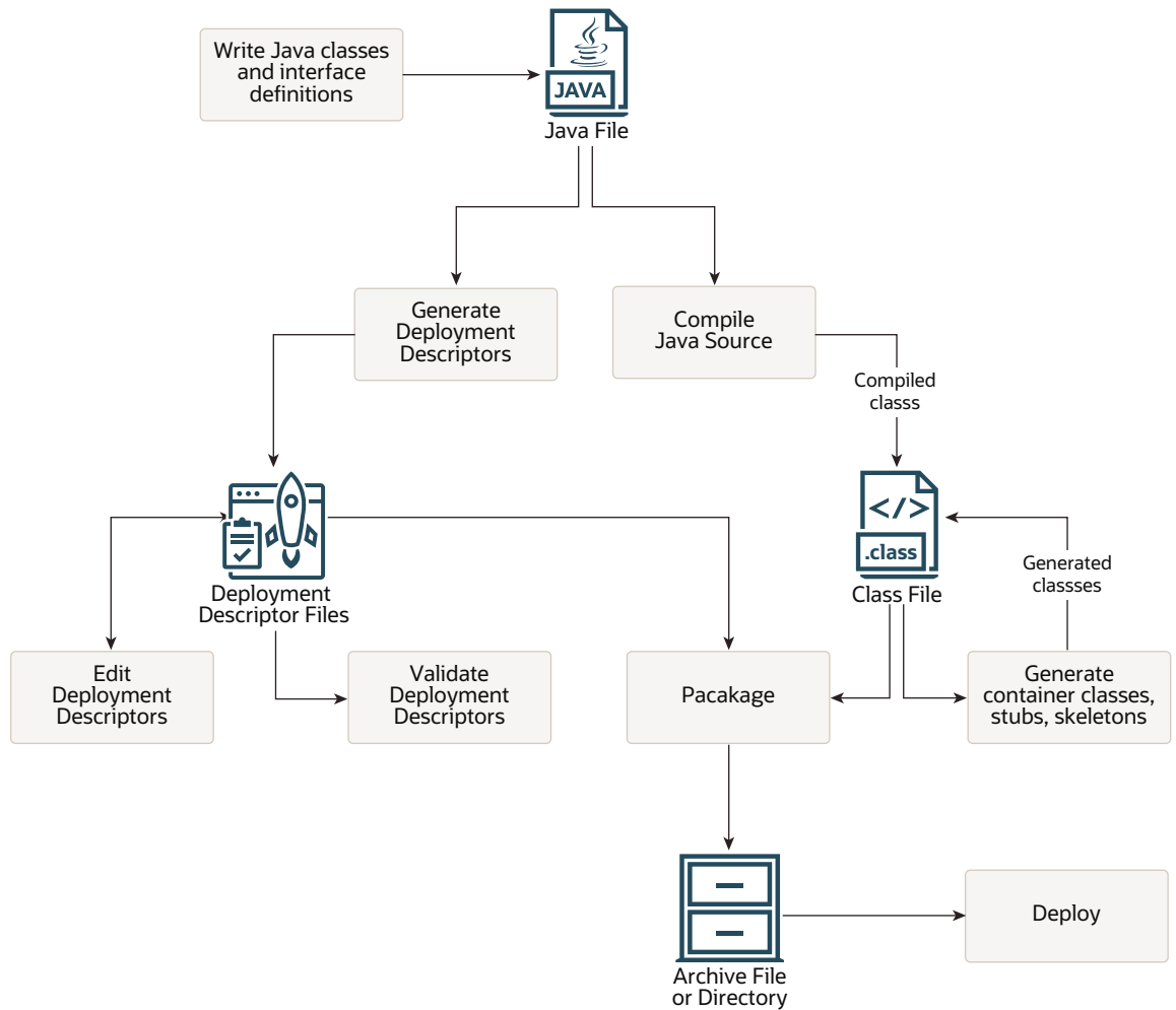
Figure 4-1 EJB Development Process Overview
