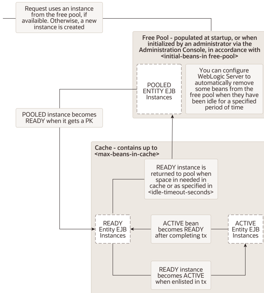
Figure 6-1 Entity Bean Life Cycle
