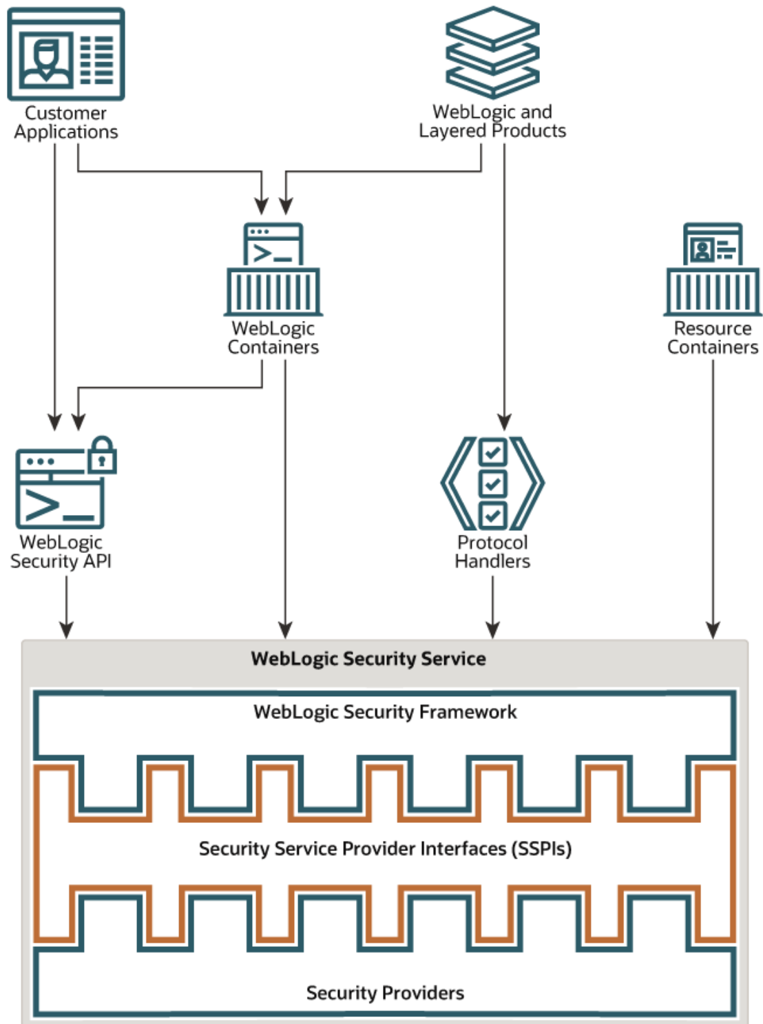
Figure 10-1 WebLogic Security Service Architecture
