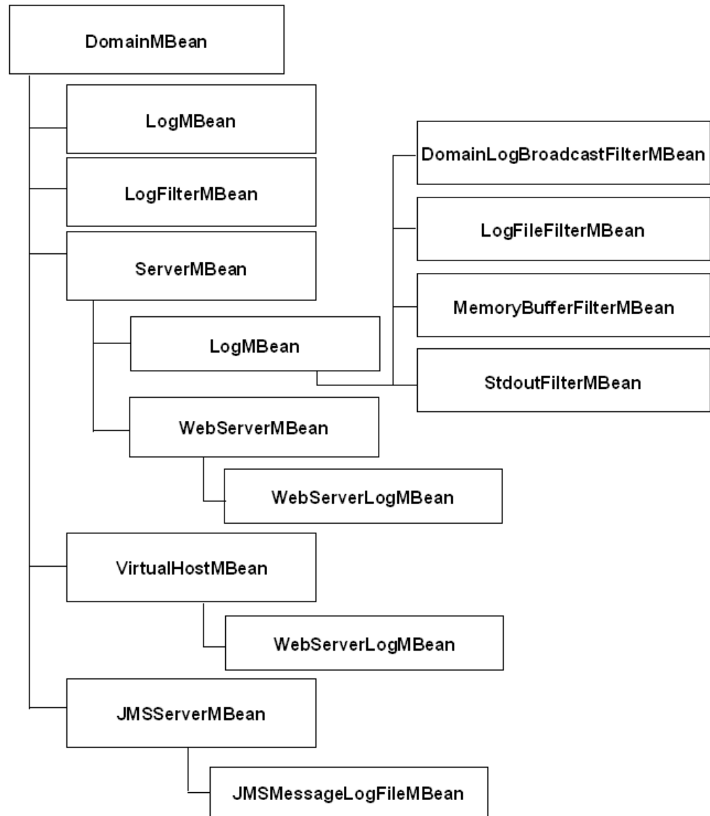
Figure 3-1 Logging MBeans
