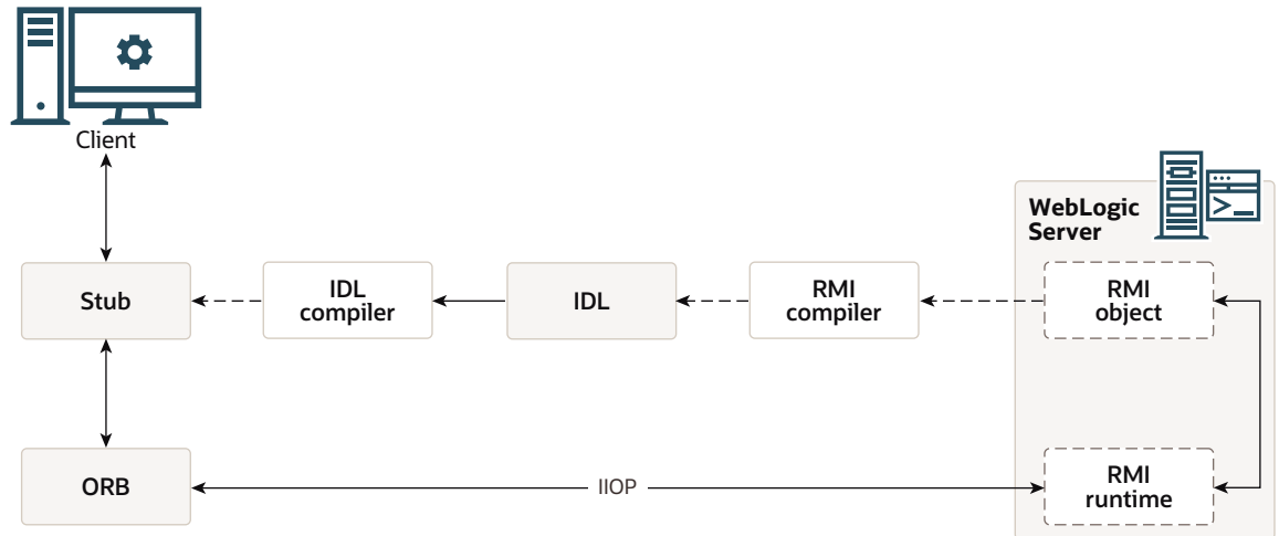
Figure 9-2 WebLogic RMI over IIOP object relationships
