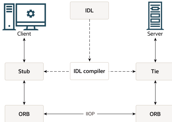
Figure 9-1 IDL Client relationships
