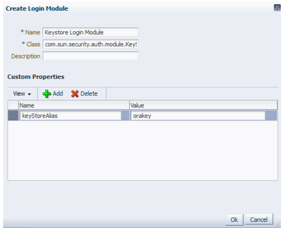
Figure 14-3 Custom Login Module Page
