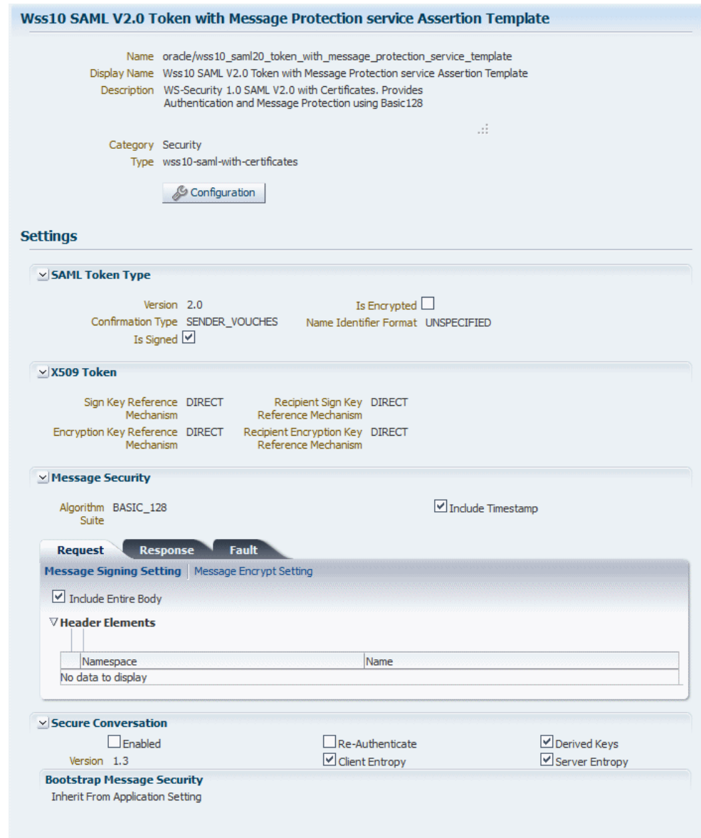
Figure 6-7 Assertion Template Details Page
