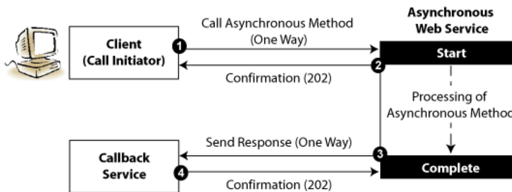
Figure 4-3 Asynchronous Web Service Client Flow
