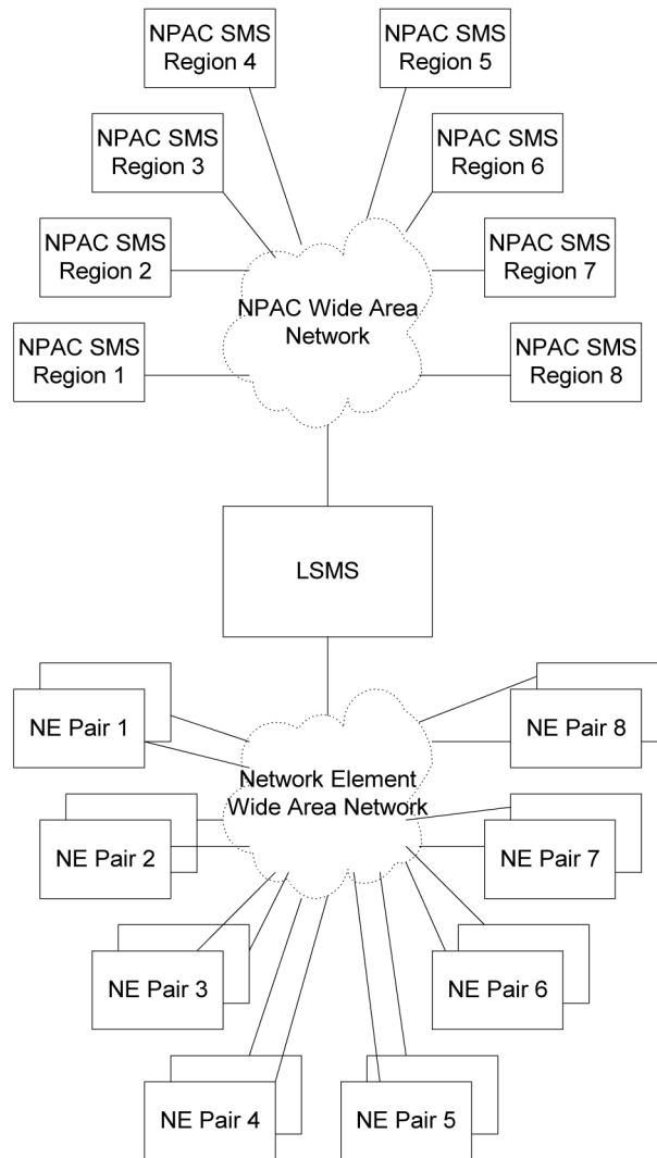
Figure 2-1 LNP Configuration
