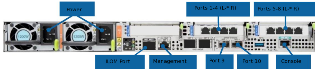
Figure 1-4 Rear Panel
