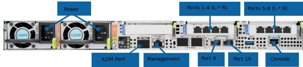
Figure 1-4 Rear Panel
