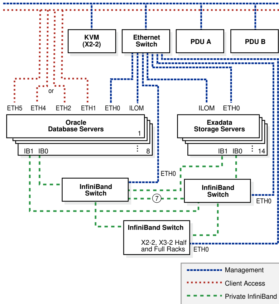
Figure 2-3 Network for Oracle Exadata Database Machine X6-2, X5-2, X4-2, X3-2, and X2-2 with Bonded Client Access
