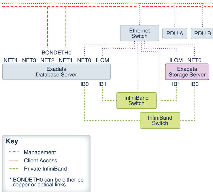
Figure 2-2 Network for Oracle Exadata Database Machine X7-2 and X8-2 with Bonded Client Access
