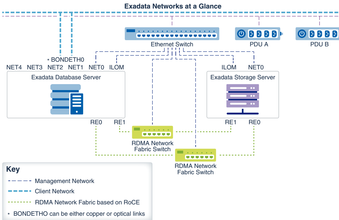
Figure 2-1 Network for Oracle Exadata Database Machine X8M-2 with Bonded Client Access
