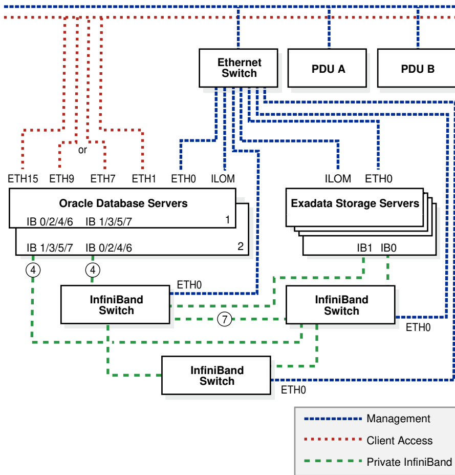
Figure 2-5 Network Diagram for Oracle Exadata Database Machine X3-8 Full Rack, and Oracle Exadata Database Machine X2-8 Full Rack with Bonded Client Access
