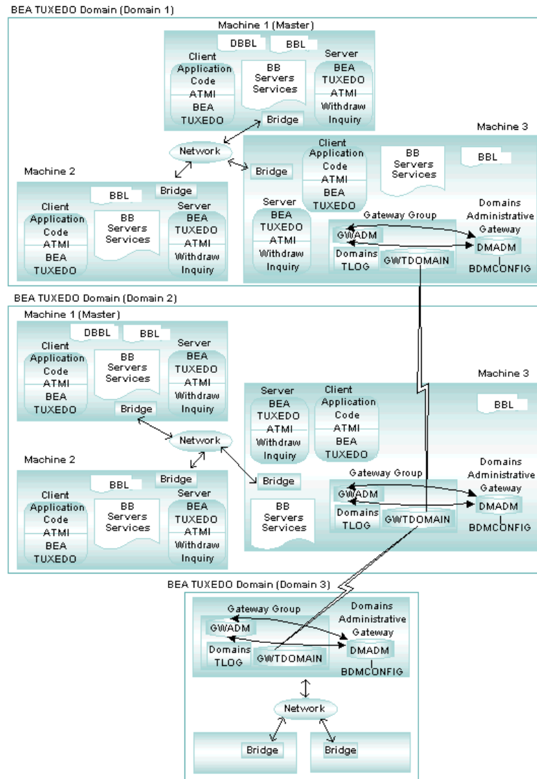
Figure 3-9 Domains Configuration
