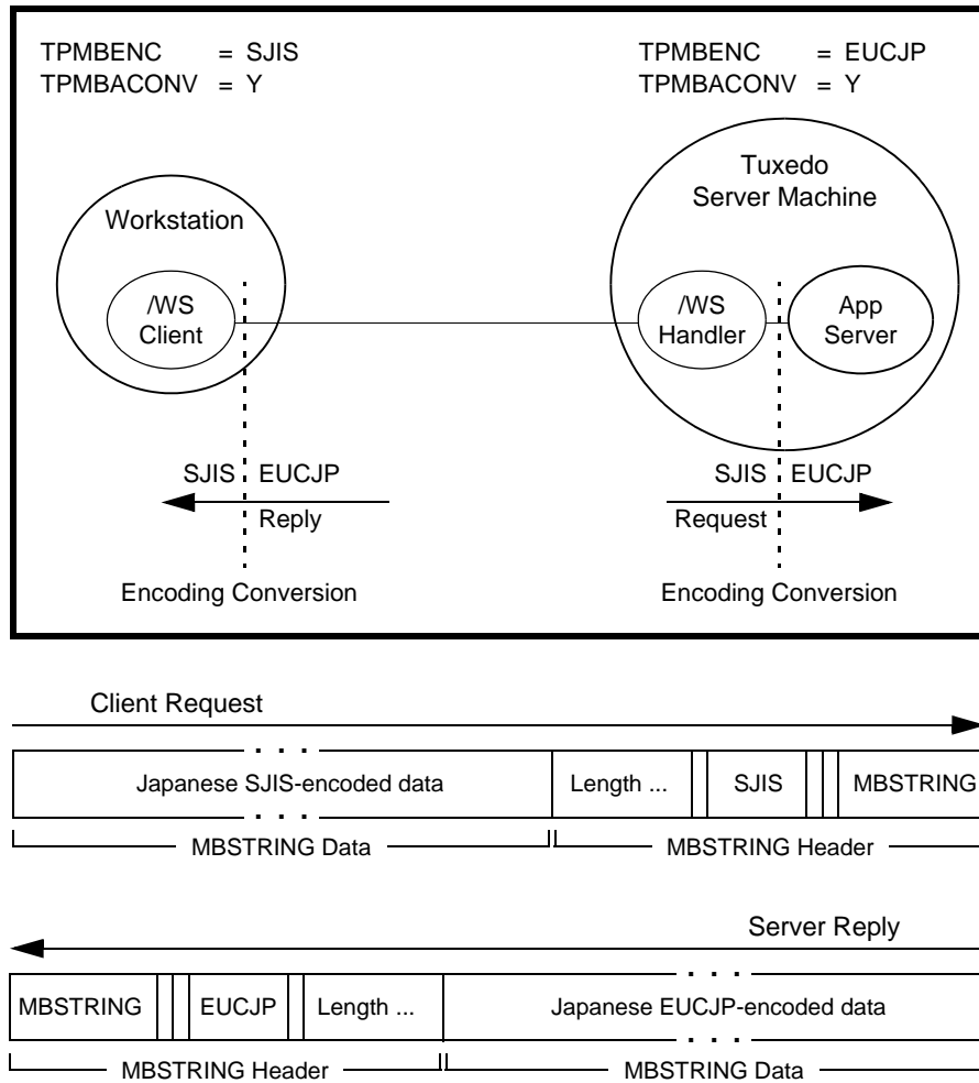
Figure 3-1 Encoding Conversion Using MBSTRING Buffers—Example
