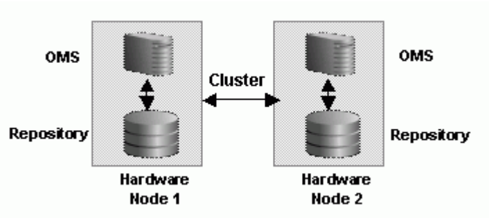
Figure 17-5 Management Service and Management Repository on Same Hardware
