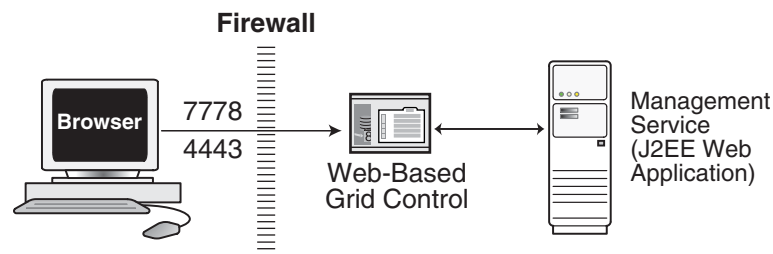
Figure 20–2 Firewall Between Your Browser and the Grid Control Console
