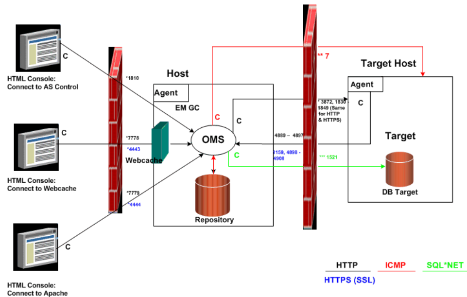
Figure 20–1 Firewall Port Requirements (Default)
