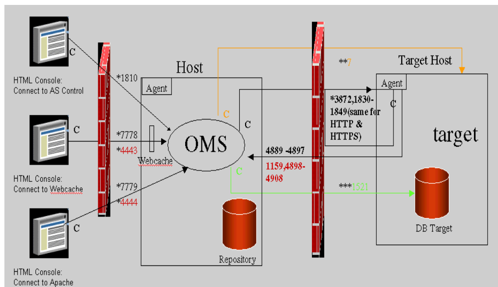
Figure G-1 Enterprise Manager Firewall Port Requirements
