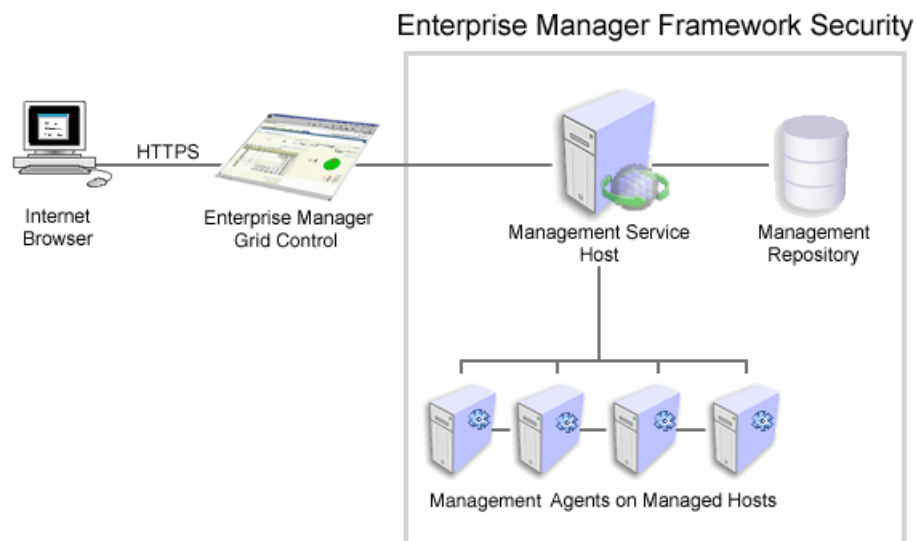
Figure 19–1 Enterprise Manager Framework Security
