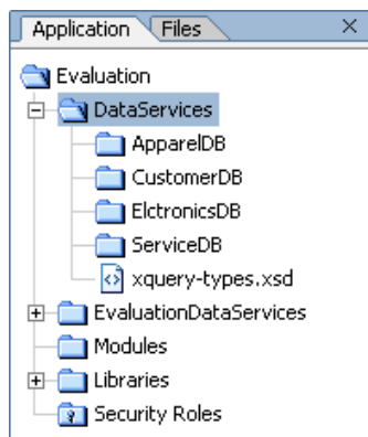
Figure 2-4 Project Sub-Folders
