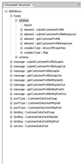
Figure 9-5 Document Structure
