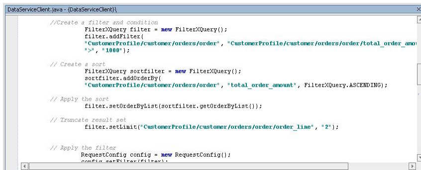
Figure 11-5 Truncate Code
