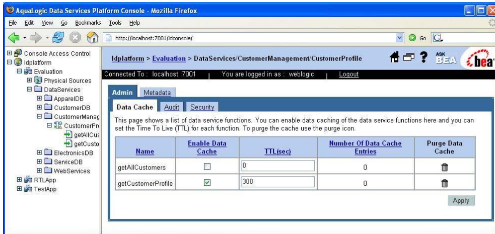
Figure 15-3 Setting TTL
