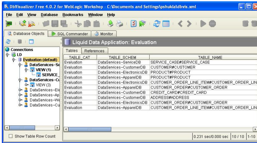
Figure 12-3 Tables
