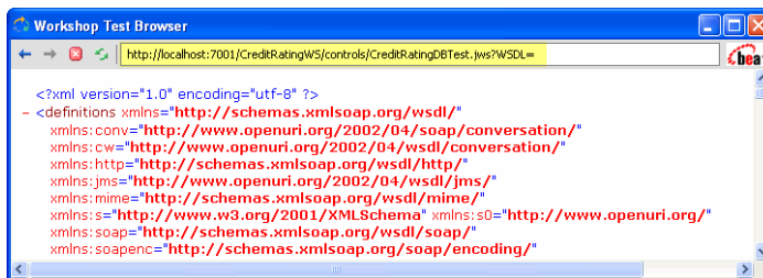
Figure 6-7 WSDL URI
