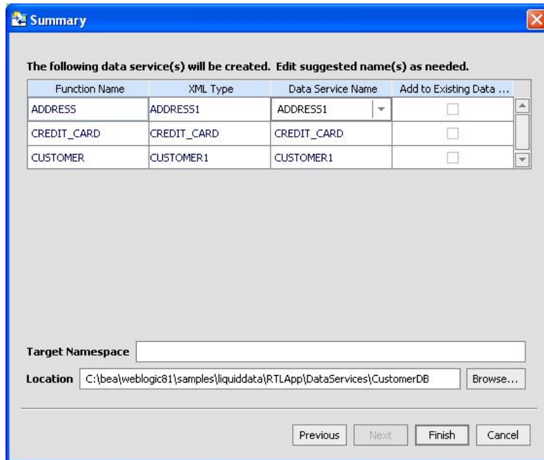
Figure 2-8 Summary
