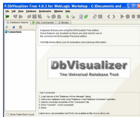
Figure 12-1 DBVisualizer Interface
