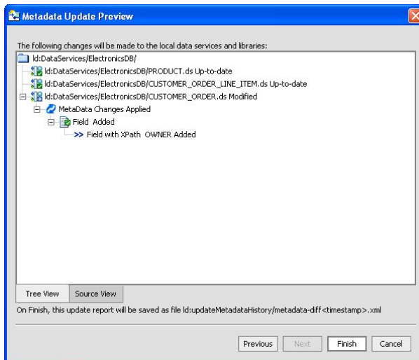
Figure 14-11 Synchronization Preview
