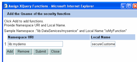
Figure 30-7 QName Information
