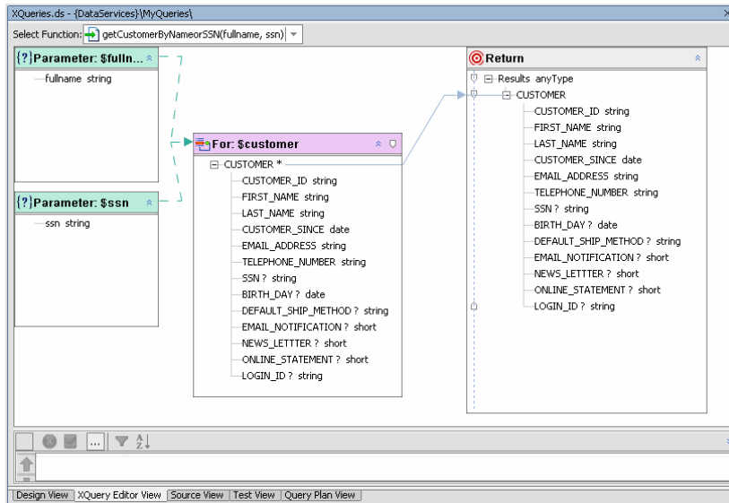
Figure 19-9 XQuery Editor View of String Function
