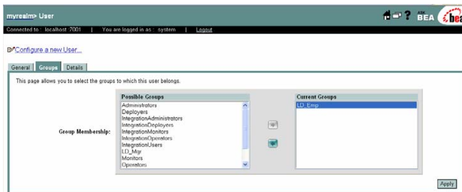
Figure 30-3 Group Assignment Page for Bob
