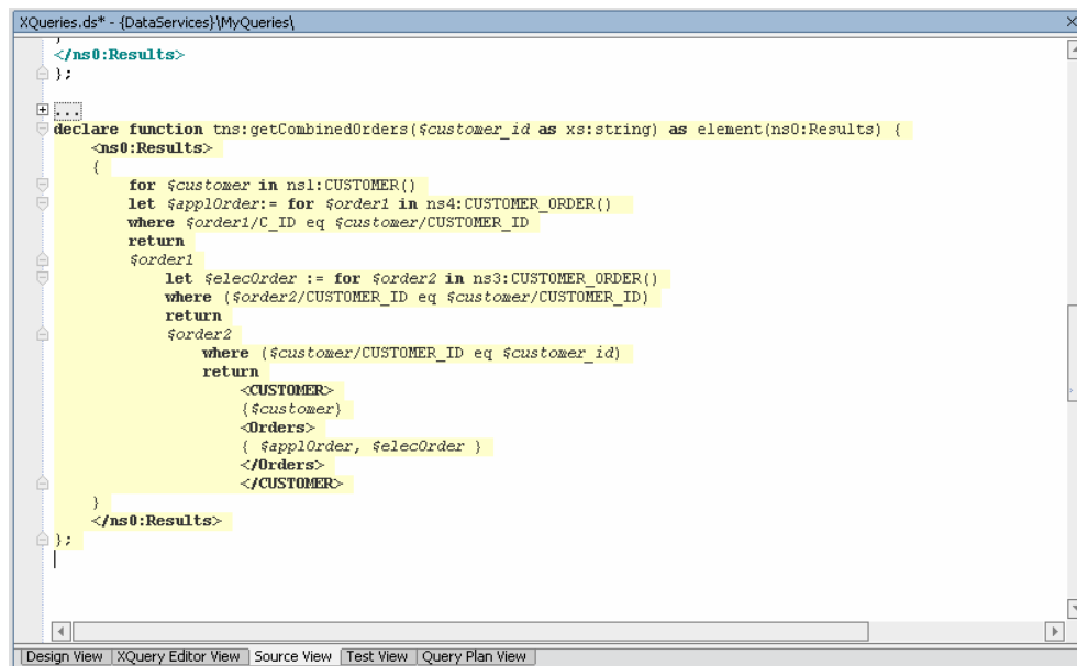
Figure 19-23 Source View for Union and Concatenation Function
