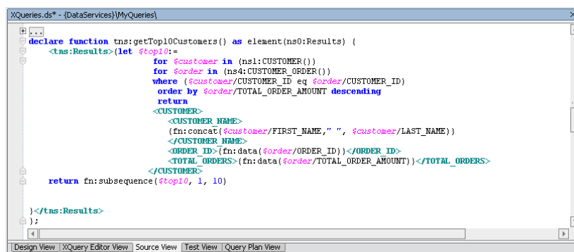
Figure 19-14 Source Code for Inner Join and Top N Function
