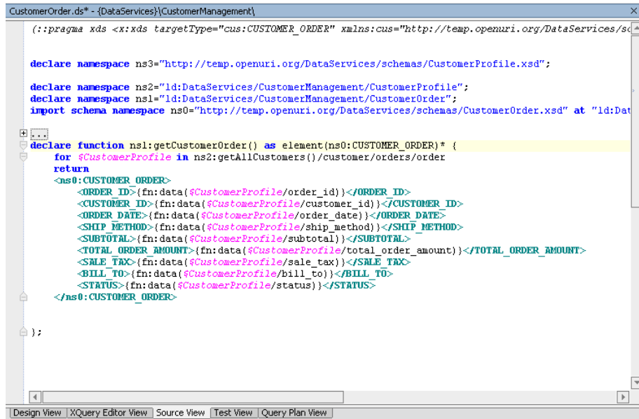
Figure 27-4 Source View of Vertical File Unfolding Function
