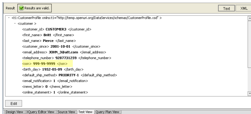
Figure 35-5 Test View of Protected SSN
