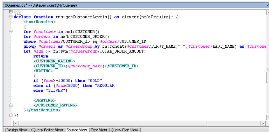
Figure 19-20 Source View of If-Then-Else Function
