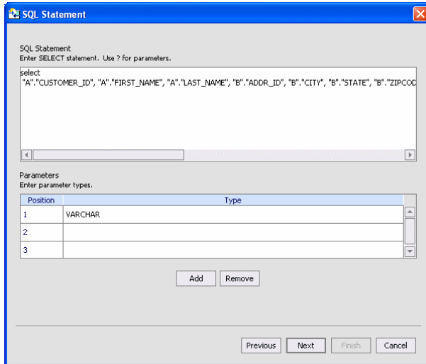
Figure 22-1 SQL Statement
