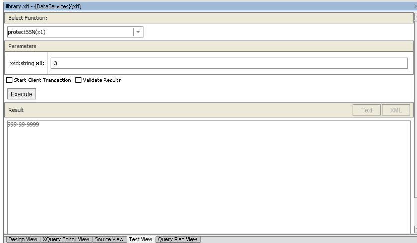
Figure 35-4 XQuery Function Library Test
