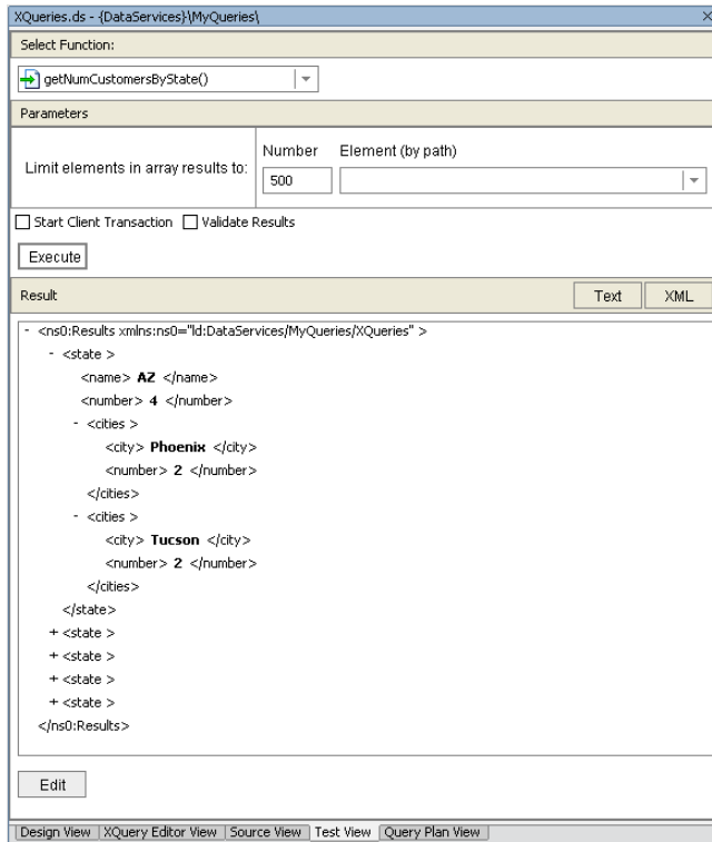
Figure 19-19 Test View of Multi-Level Group By Function
