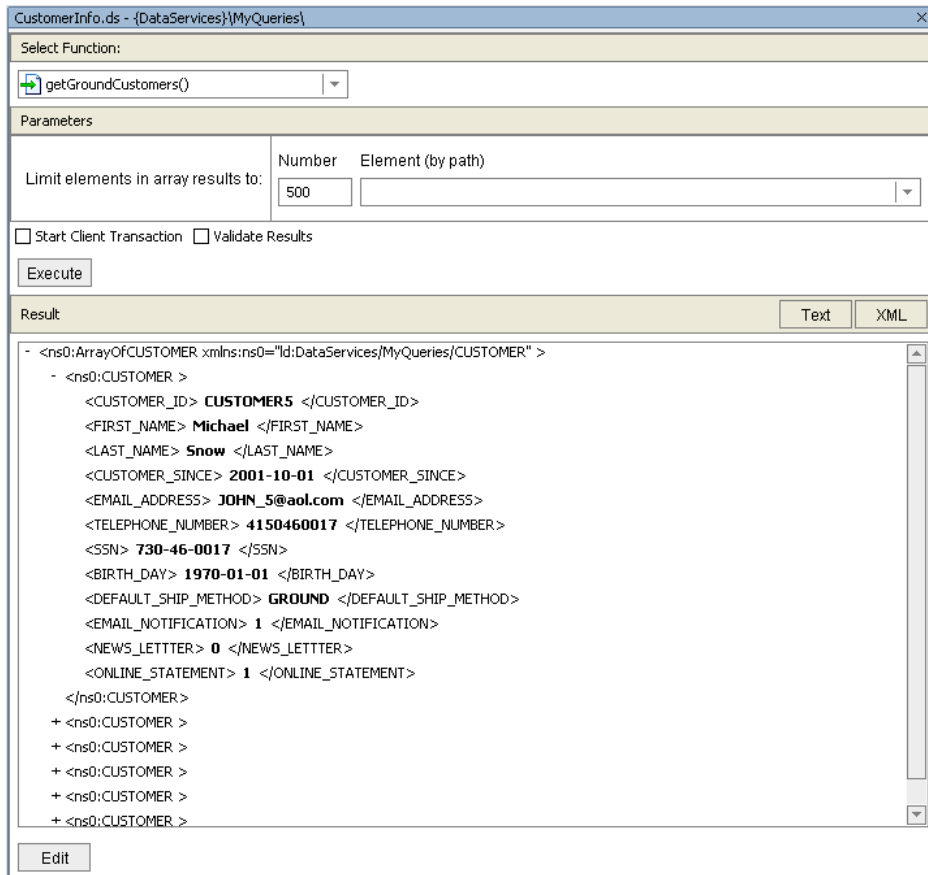
Figure 18-27 Test Results of a Constant Expression
