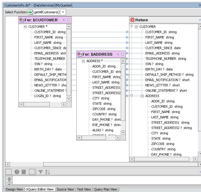
Figure 18-4 Overwrite Mapping
