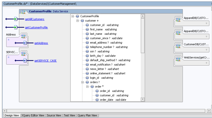
Figure 20-8 New Functions
