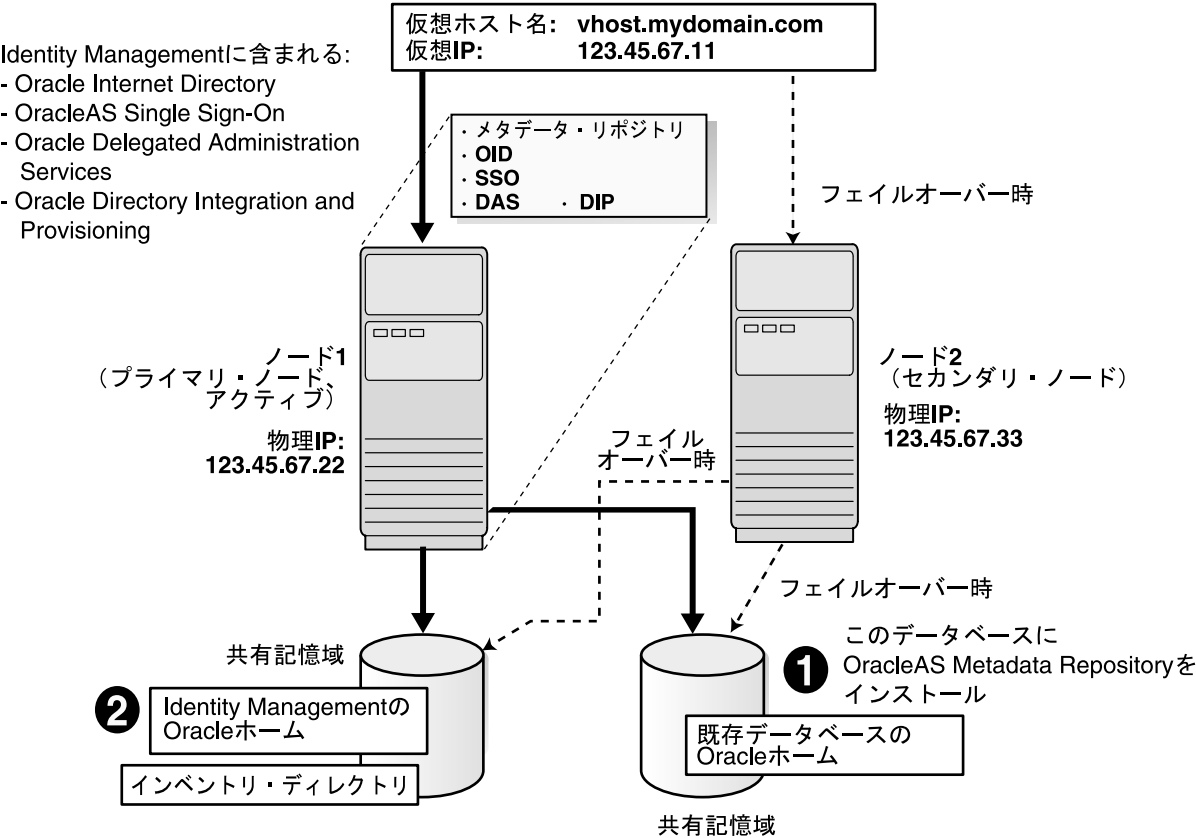
図 11-3 OracleAS Cold Failover Cluster (Oracle Identity Management) 構成
