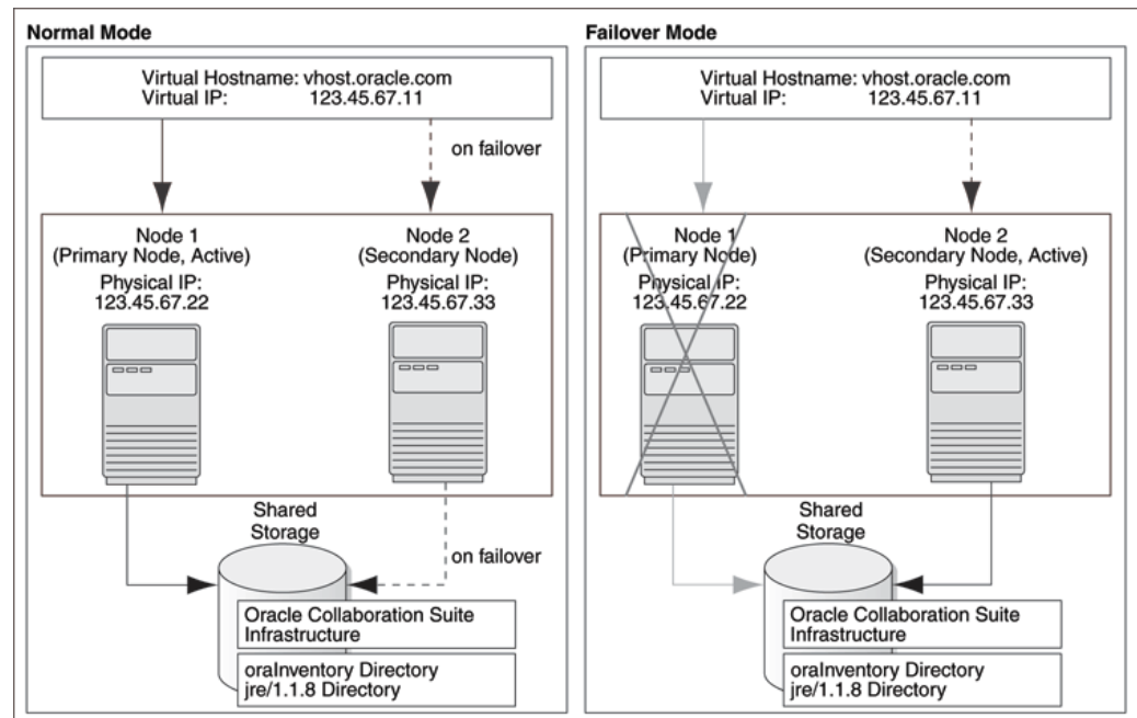
Figure 10–4 Oracle Calendar High Availability Configuration
