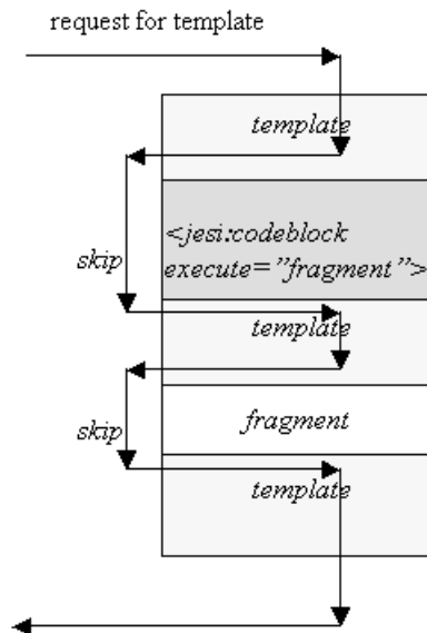
Figure 6–4 JESI codeblock Fragment Execution with Request for Template
