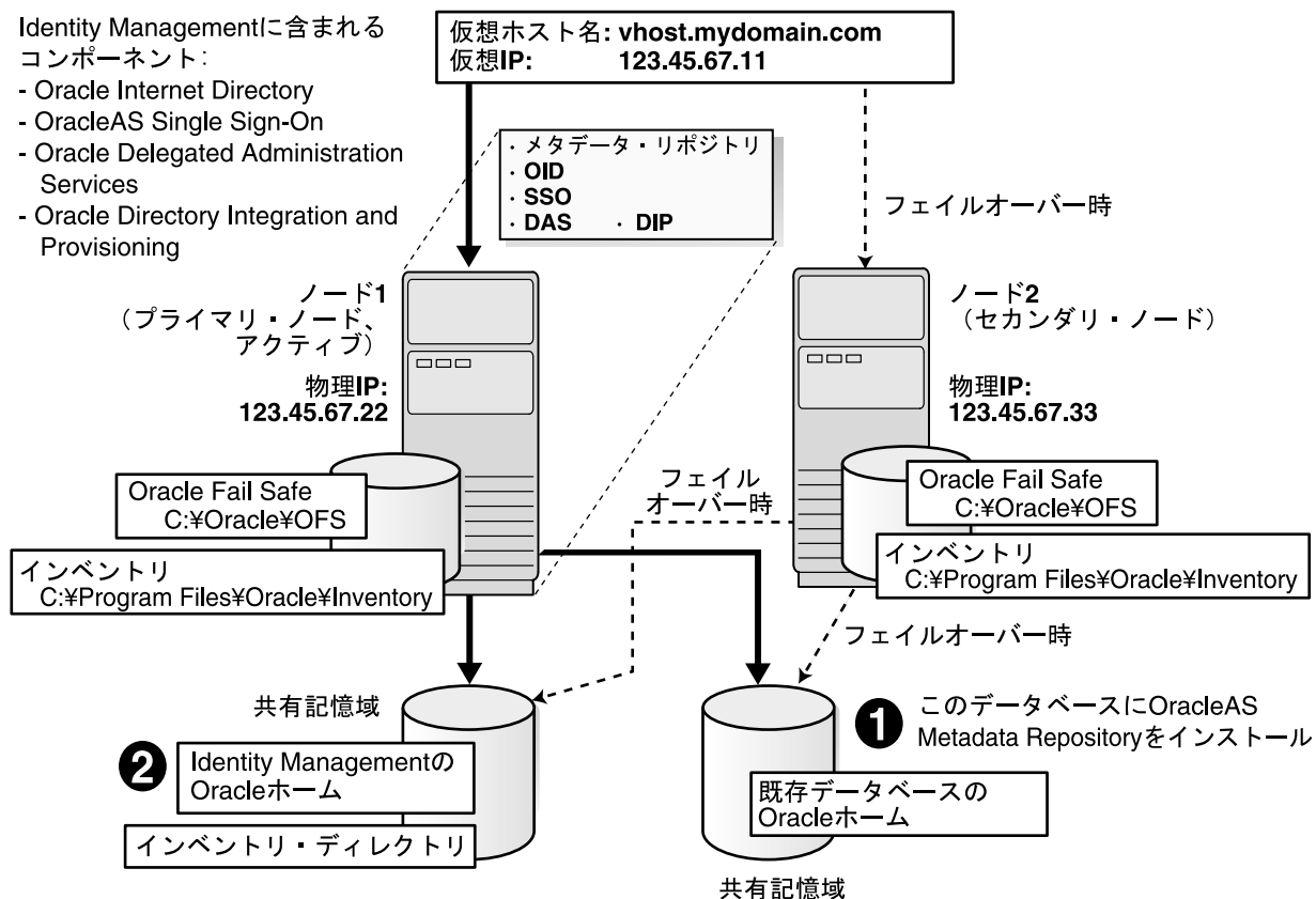
图 8-19 OracleAS Cold Failover Cluster (Identity Management) 構成
