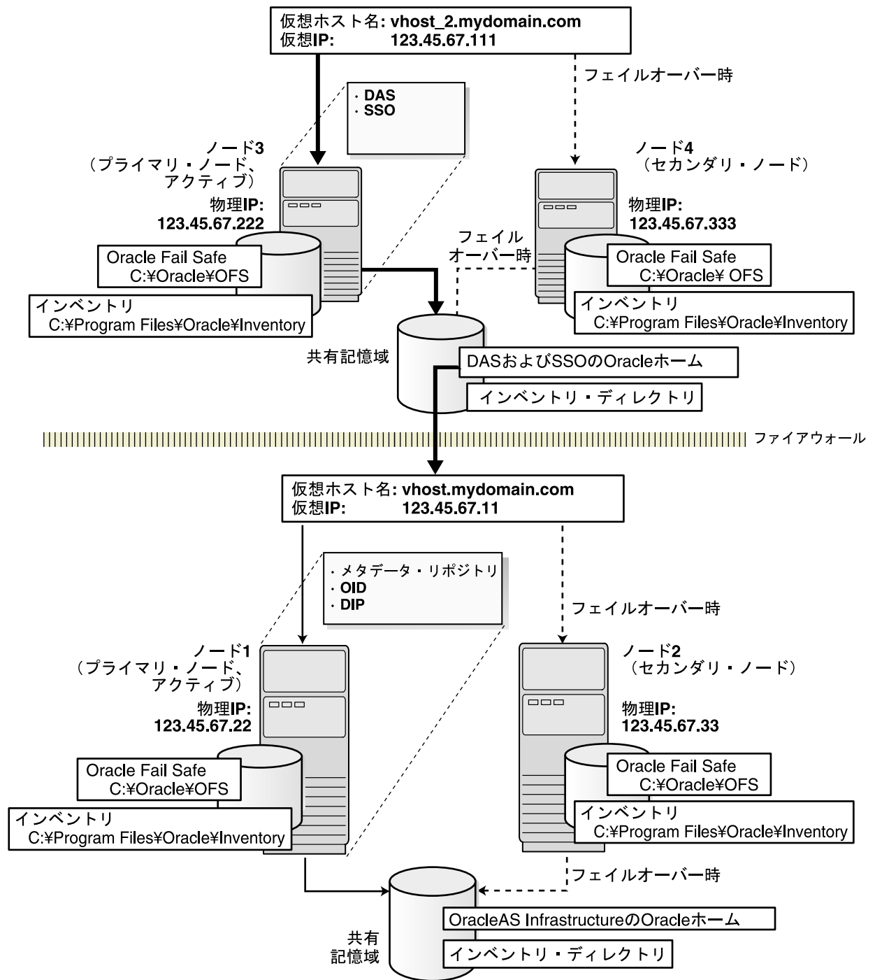
図 8-25 Cold Failover Cluster の Oracle Delegated Administration Services および OracleAS Single Sign-On
