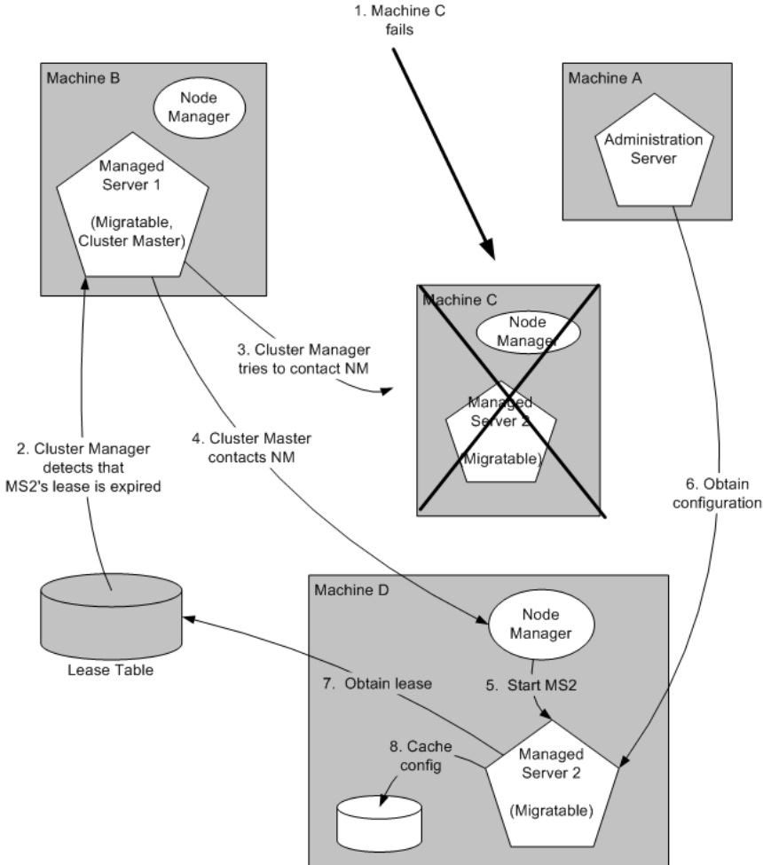
Figure 7-2 Automatic Migration of a Failed Server
