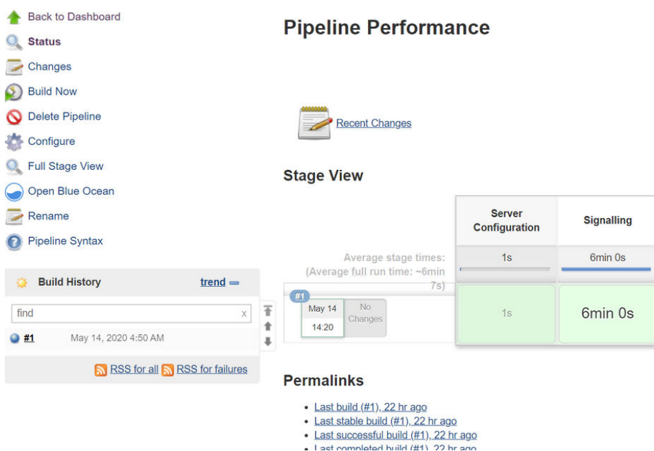
Figure 3-7 Performance Build
