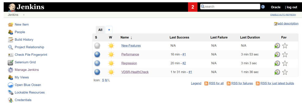
Figure 3-4 Jenkins GUI
