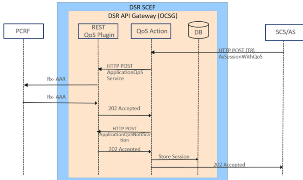
Figure 2-52 AS Session Setup
