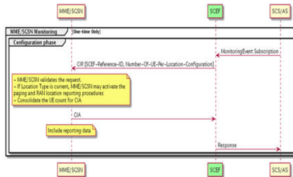
Figure 2-11 Monitoring Event Subscription Request to MME/SGSN
