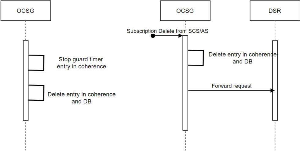
Figure 2-21 Delete Guard Timer
