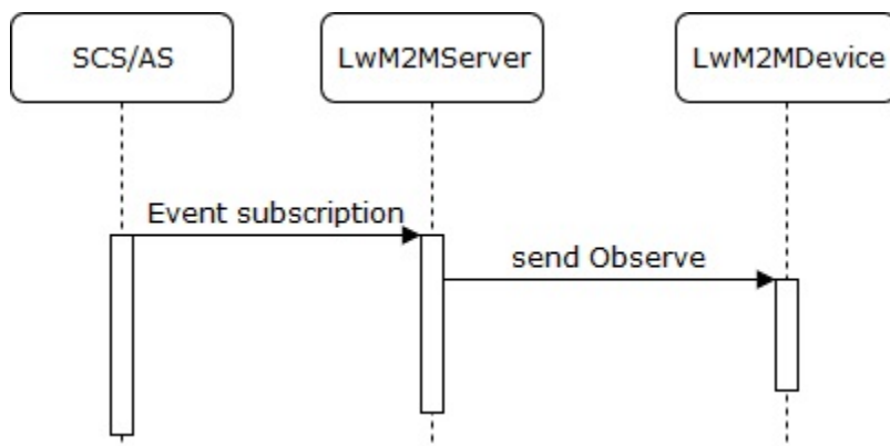
Figure 2-26 LwM2M Event Subscription Process
