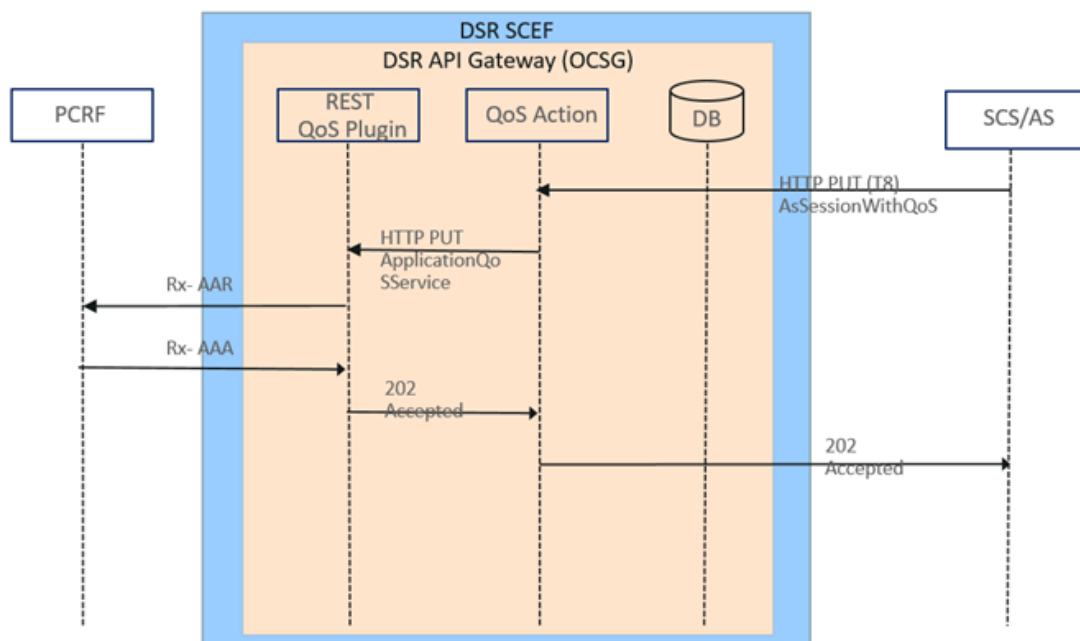
Figure 2-53 AS Session Modify
