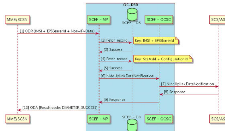
Figure 2-8 Uplink Data Notification
