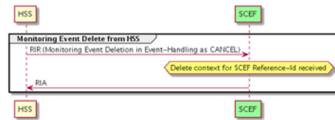
Figure 5-6 Delete Subscription from HSS
