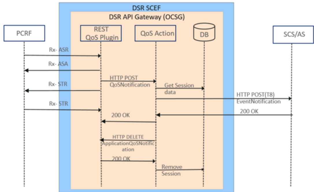
Figure 2-55 AS Session QoS Modification
