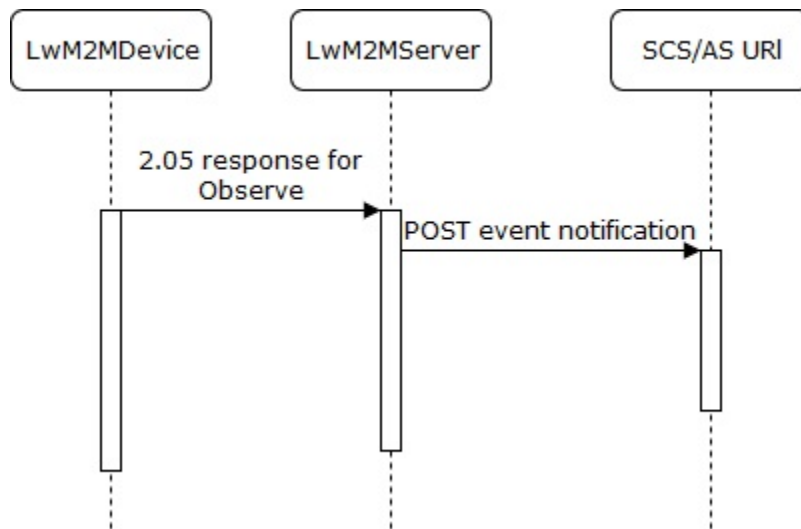
Figure 2-27 LwM2M Event Subscription Notification Process
