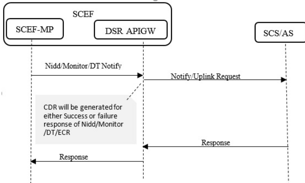
Figure 2-50 API-Based Charging for Notification Events
