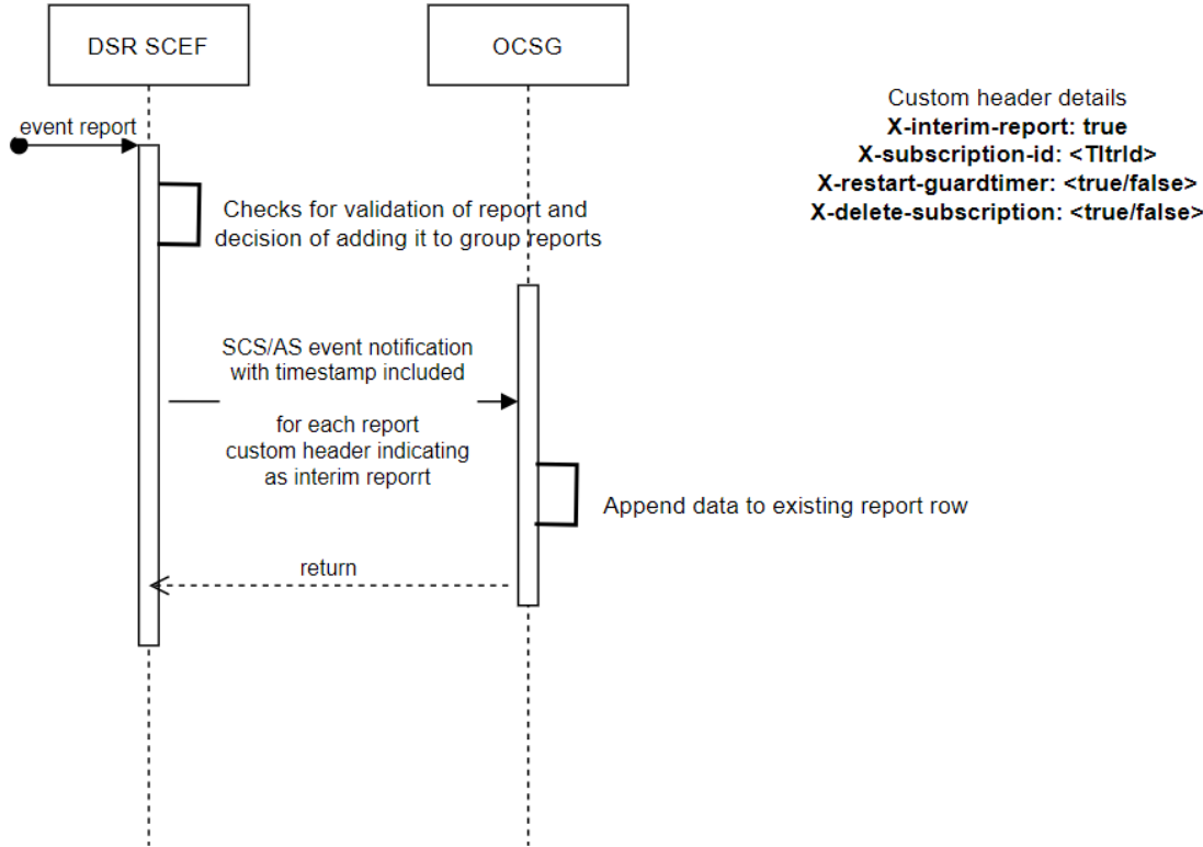
Figure 2-19 Handling event reports
