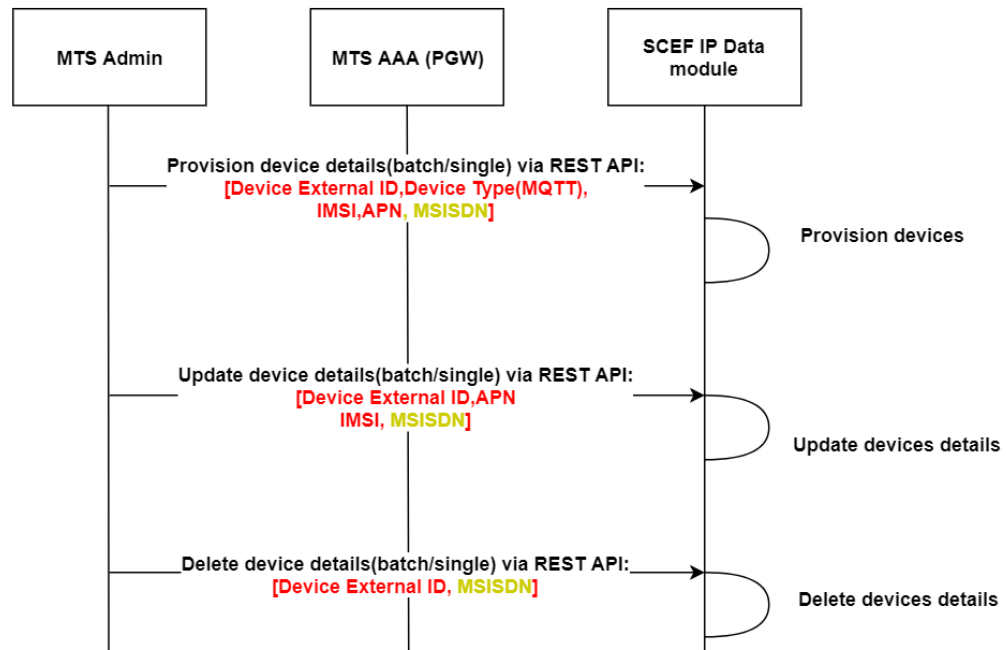
Figure 2-46 SCEF MQTT Broker device provisioning
