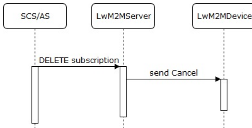
Figure 2-28 LwM2M Event Subscription Delete Process
