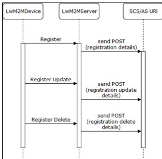
Figure 2-25 LwM2M Device Registration
