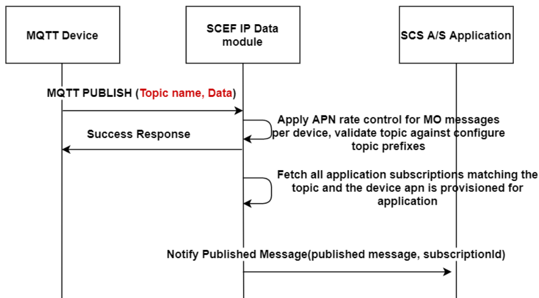
Figure 2-34 Notifications Call Flow
