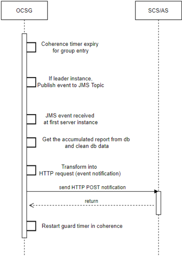
Figure 2-20 Guard timer expiry
