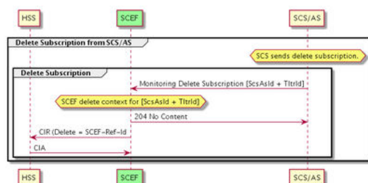
Figure 2-15 Configuration-Information-Request
