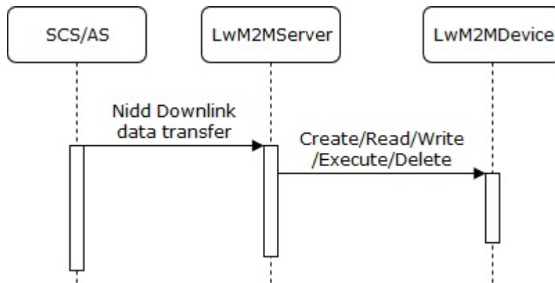
Figure 2-29 LwM2M Data Delivery Process
