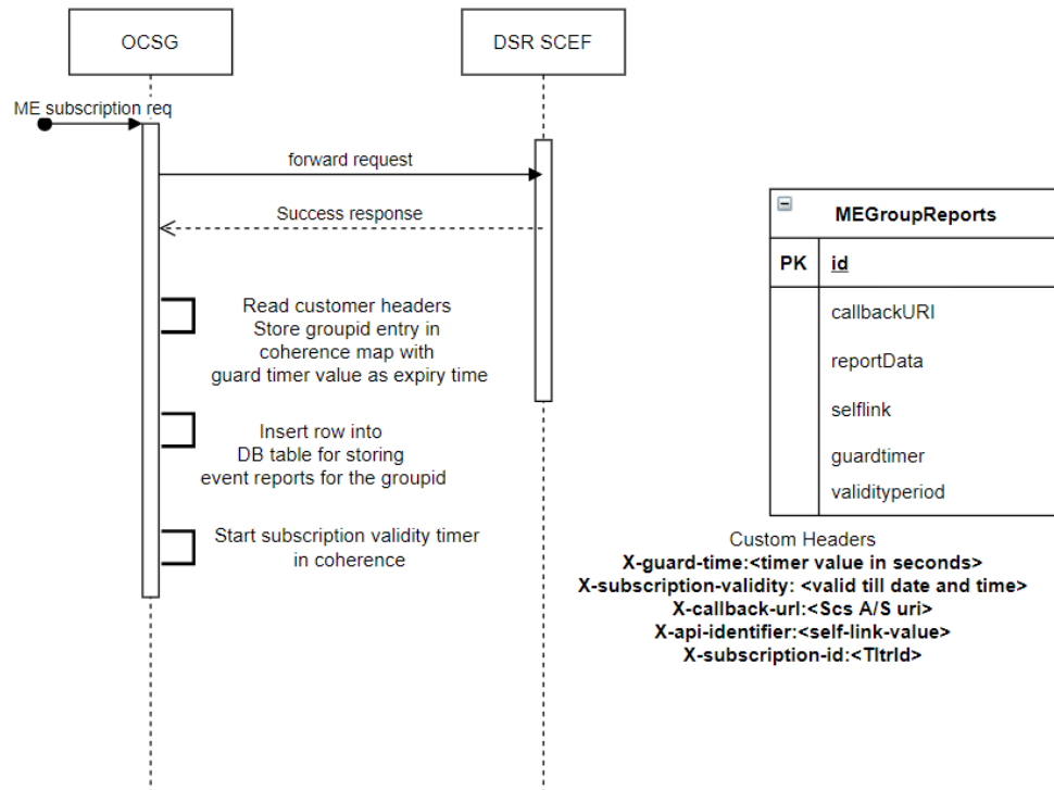
Figure 2-18 Start of Guard Timer
