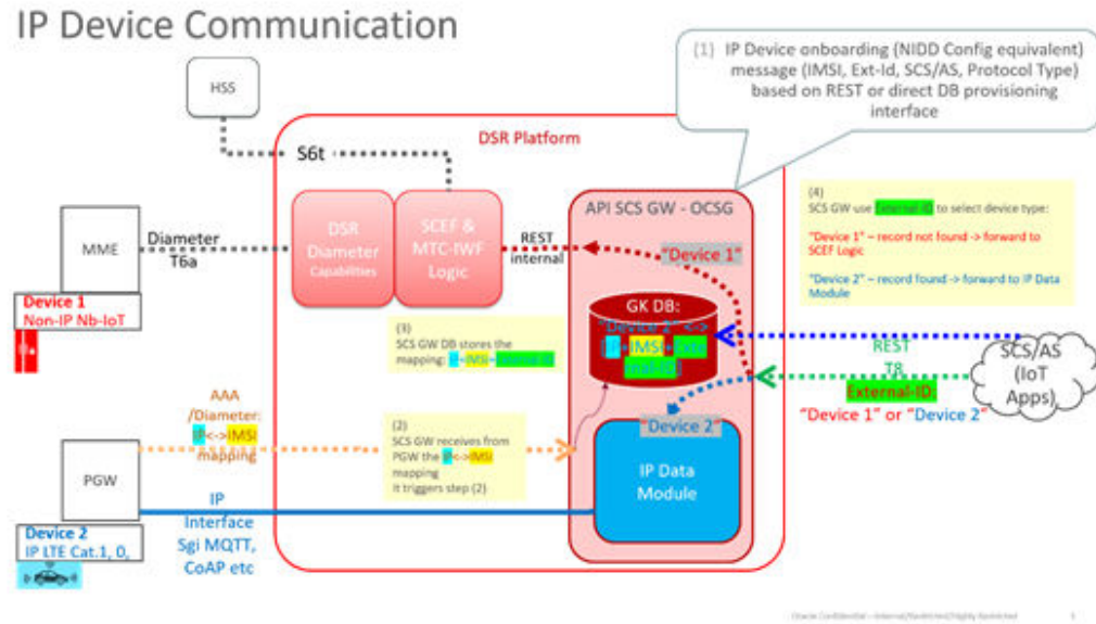
Figure 2-45 SCEF MQTT Broker - AAA Server Integration
