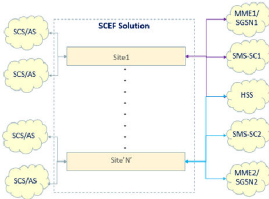
Figure 2-1 DSR-SCEF Interconnections
