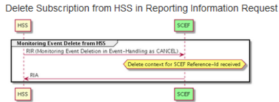
Figure 2-16 Delete Subscription from HSS
