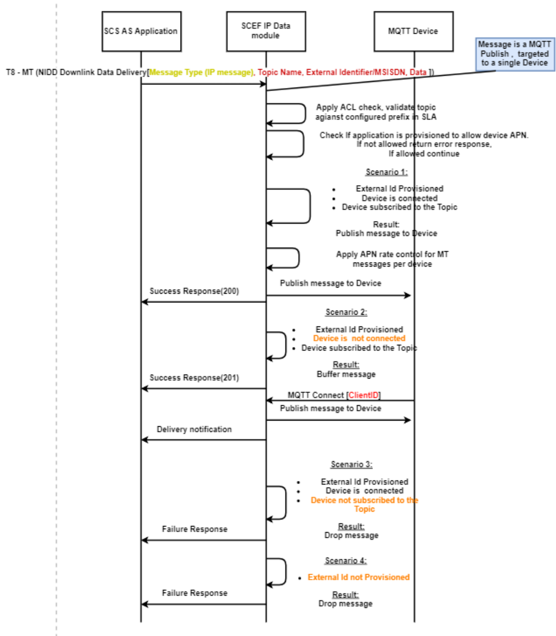
Figure 2-32 Data Delivery (Single) Call Flow
