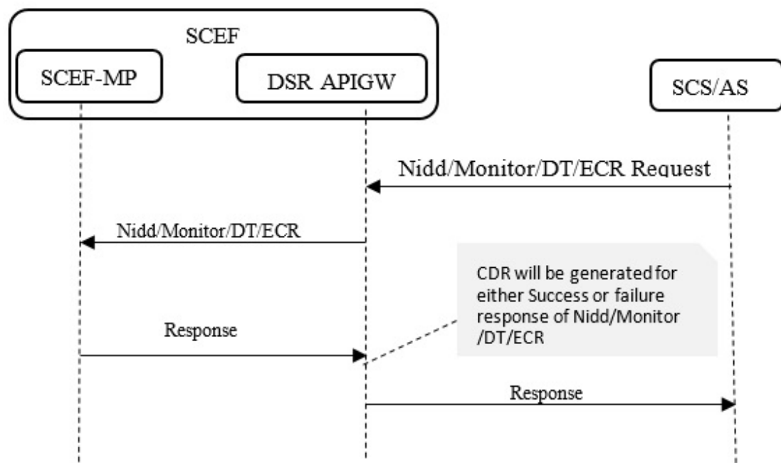
Figure 2-49 API-Based Charging for Invocation Events
