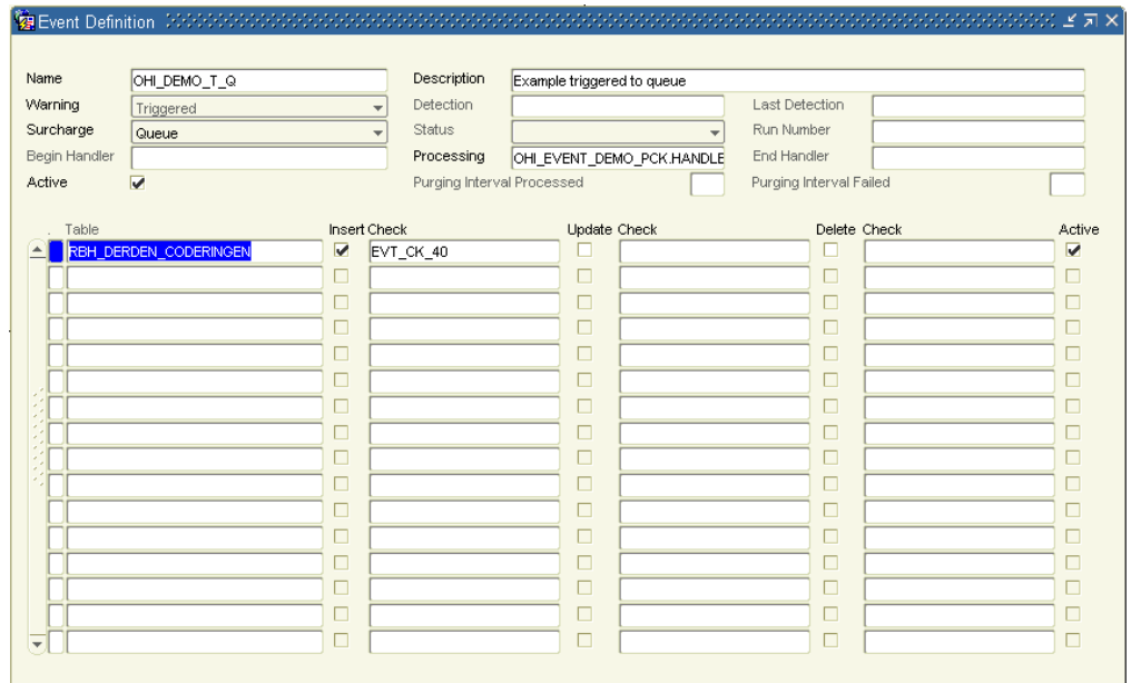
Figure 28: Add a table and evaluation function to a triggered event
