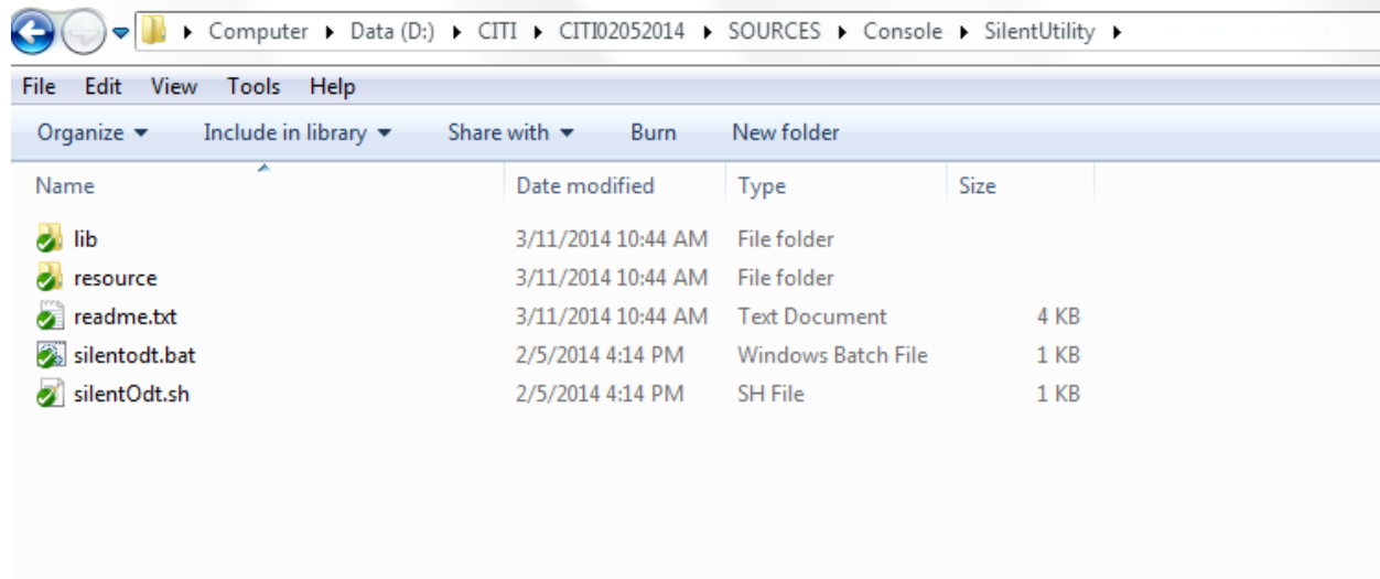
Fig 4.4.1: SilentODT Sources
