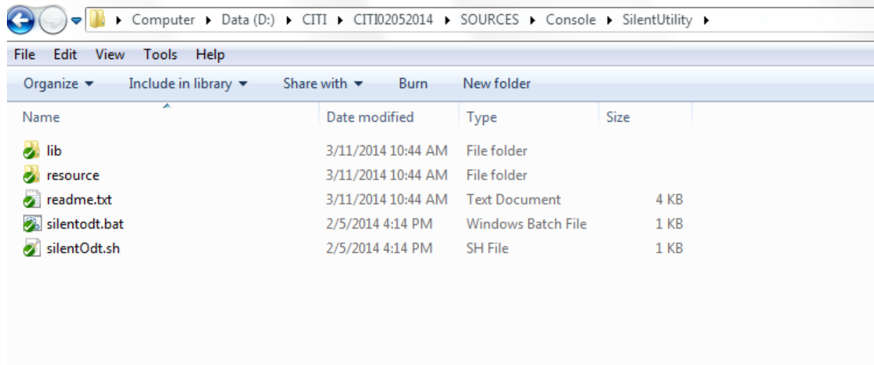
Fig 4.4.1: SilentODT Sources
