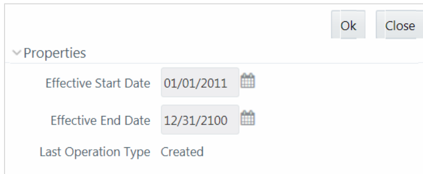
Figure 178: Properties window
