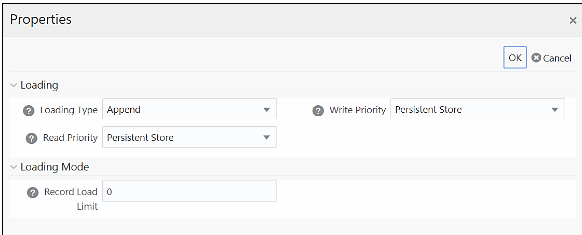
Figure 43: Properties window
