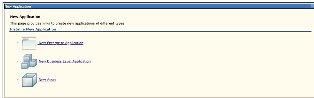
Figure 34: New Application
