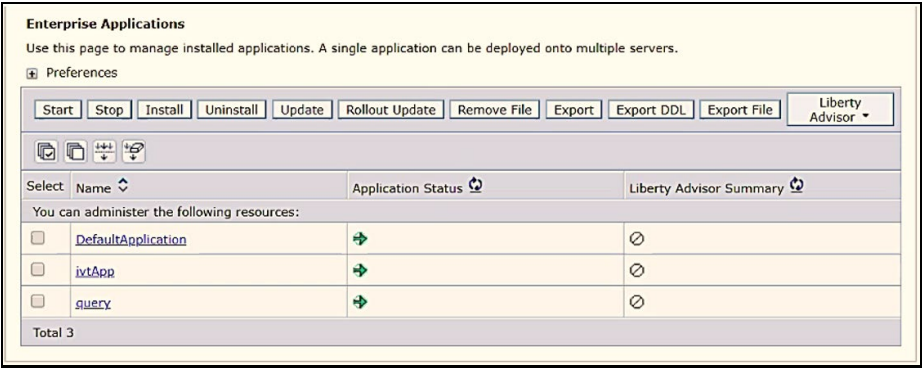
Figure 69: Enterprise Applications
