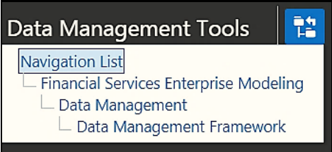
Figure 53: Navigation Submenu
