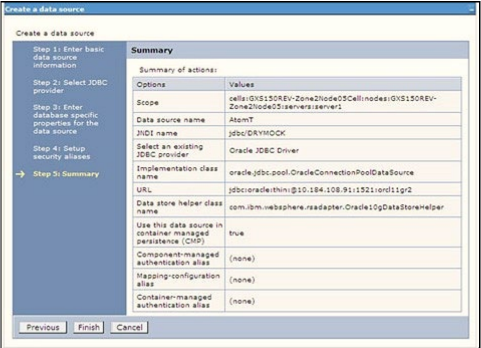
Figure 95: Summary
