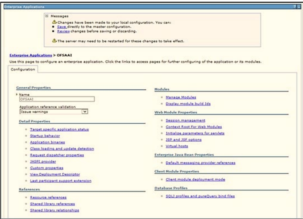
Figure 128: OFSAAI Configuration
