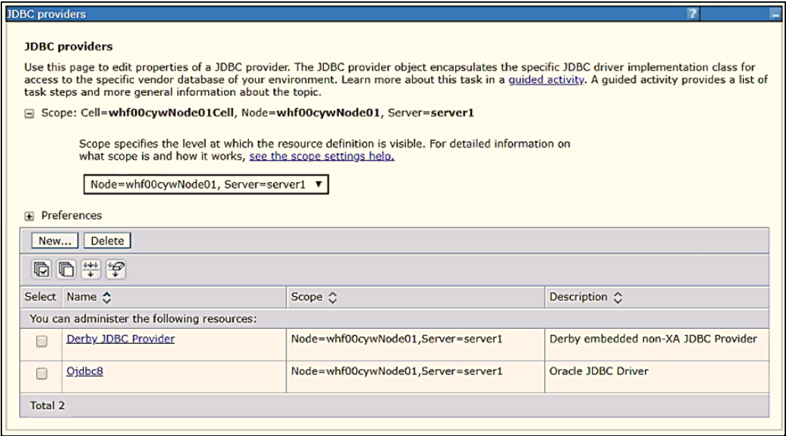
Figure 86: JDBC Providers
