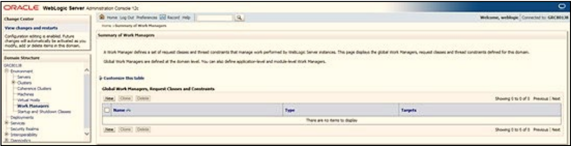
Figure 131: Work Manager
