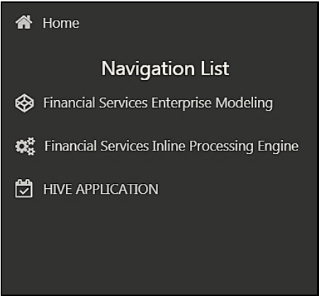
Figure 51: Navigation Drawer
