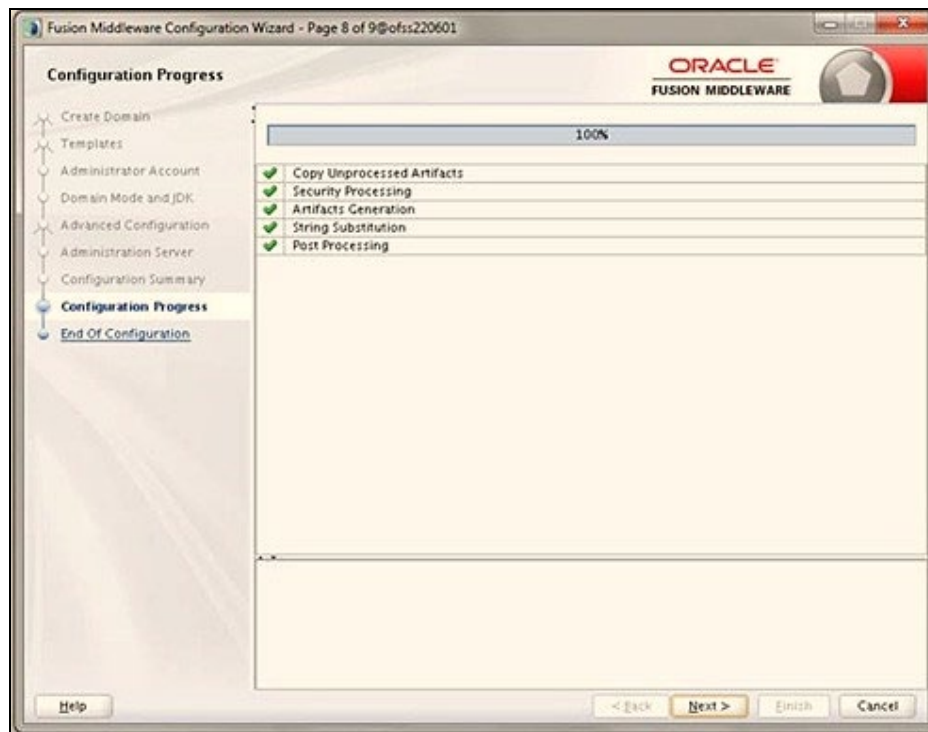
Figure 80: Creating Domain
