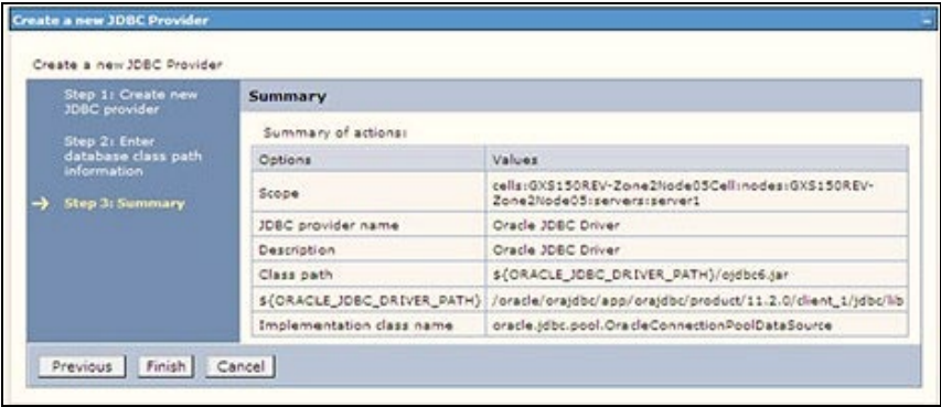
Figure 89: Summary
