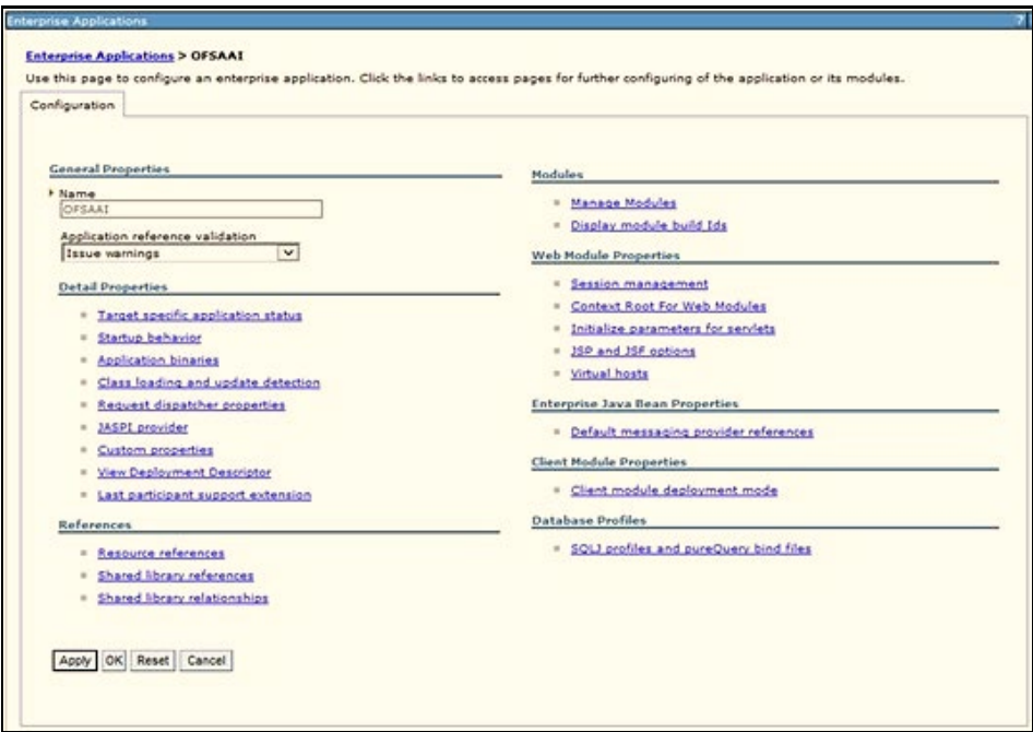
Figure 124: OFSAAI
