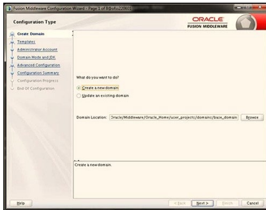
Figure 73: Configuration Type
