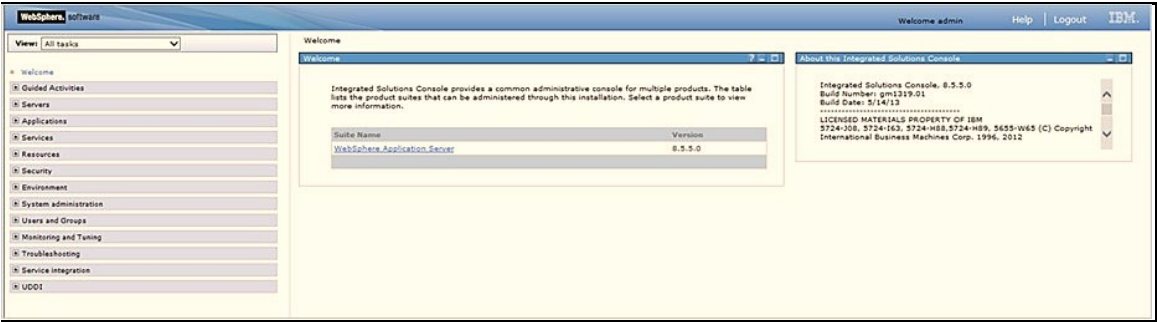
Figure 118: Home page
