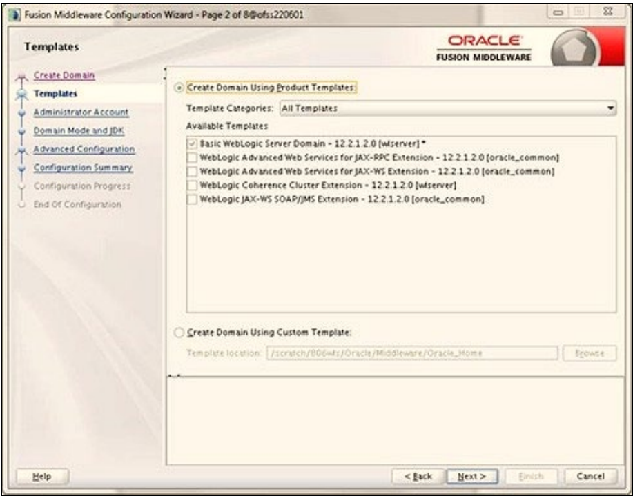
Figure 74: Templates
