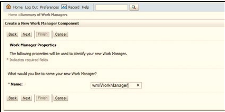
Figure 133: Work Manager
