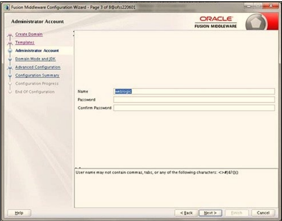
Figure 75: Administrator Account
