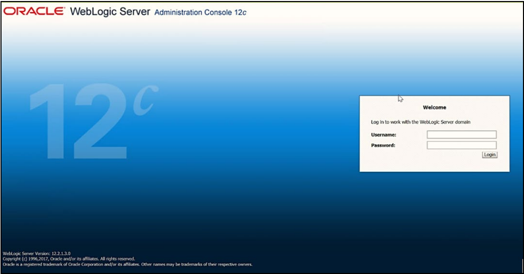
Figure 99: Welcome
