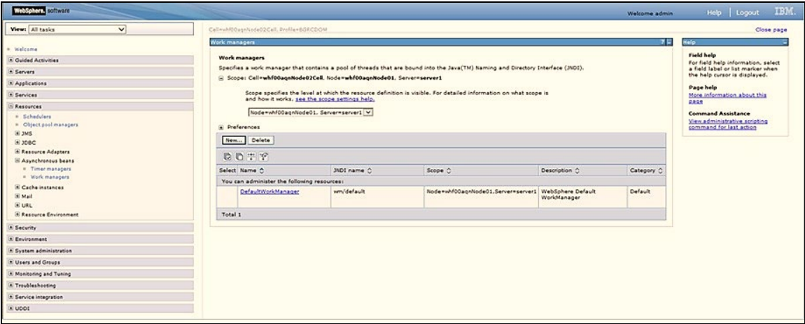
Figure 119: Work Managers
