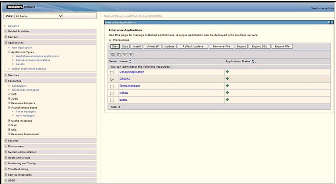
Figure 123: Enterprise Applications
