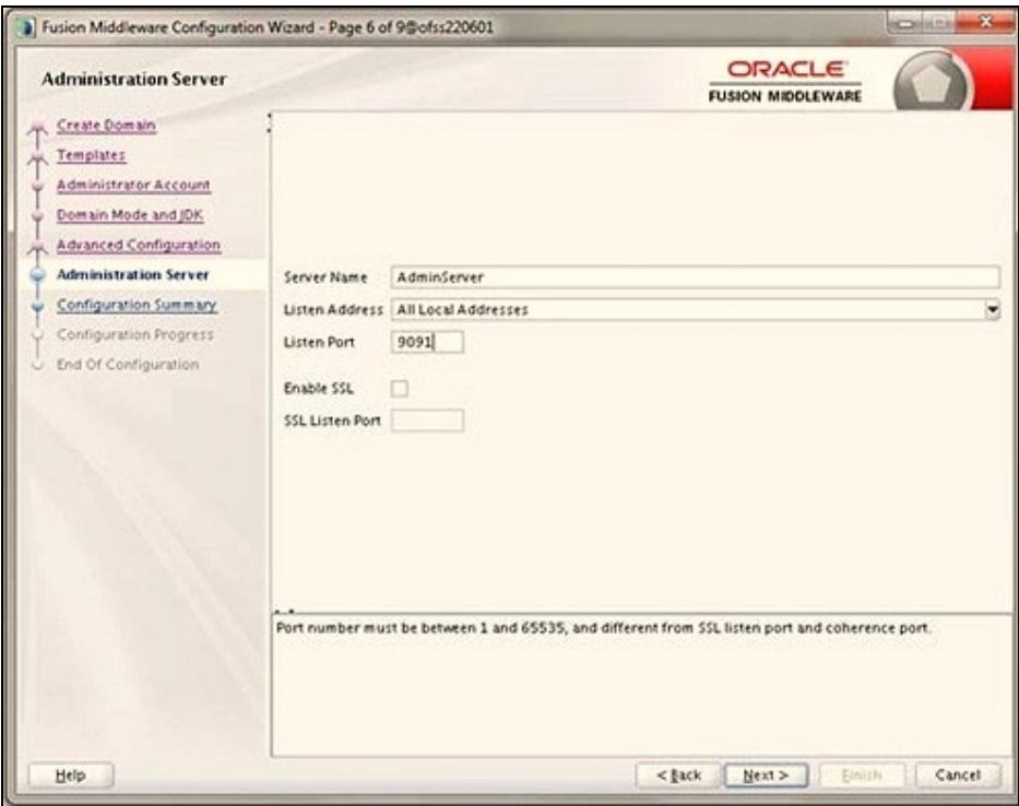
Figure 78: Administration Server
