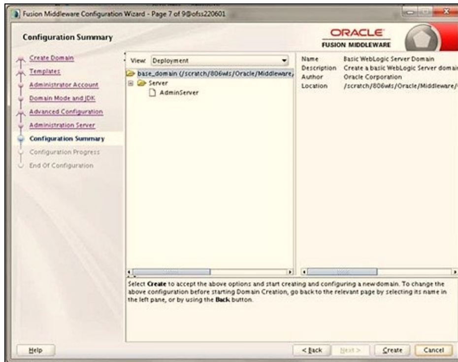
Figure 79: Configuration Summary
