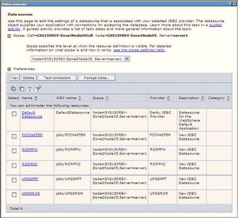
Figure 90: Data Sources
