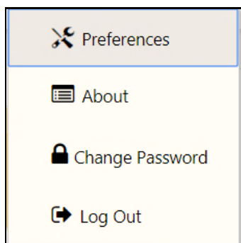
Figure 49: User Menu
