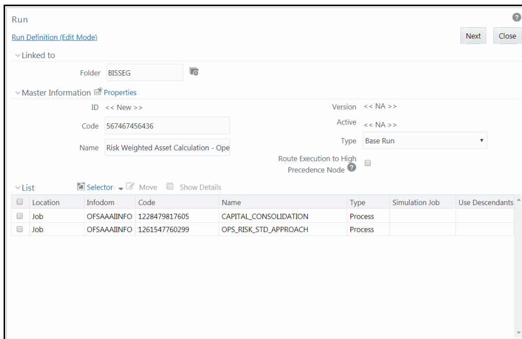
Figure 199: Run Definition (New Mode) window
