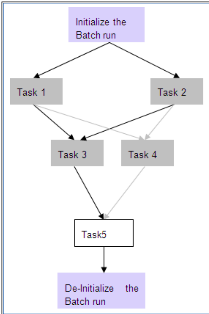
Figure 318: Illustration of Batch Execution
