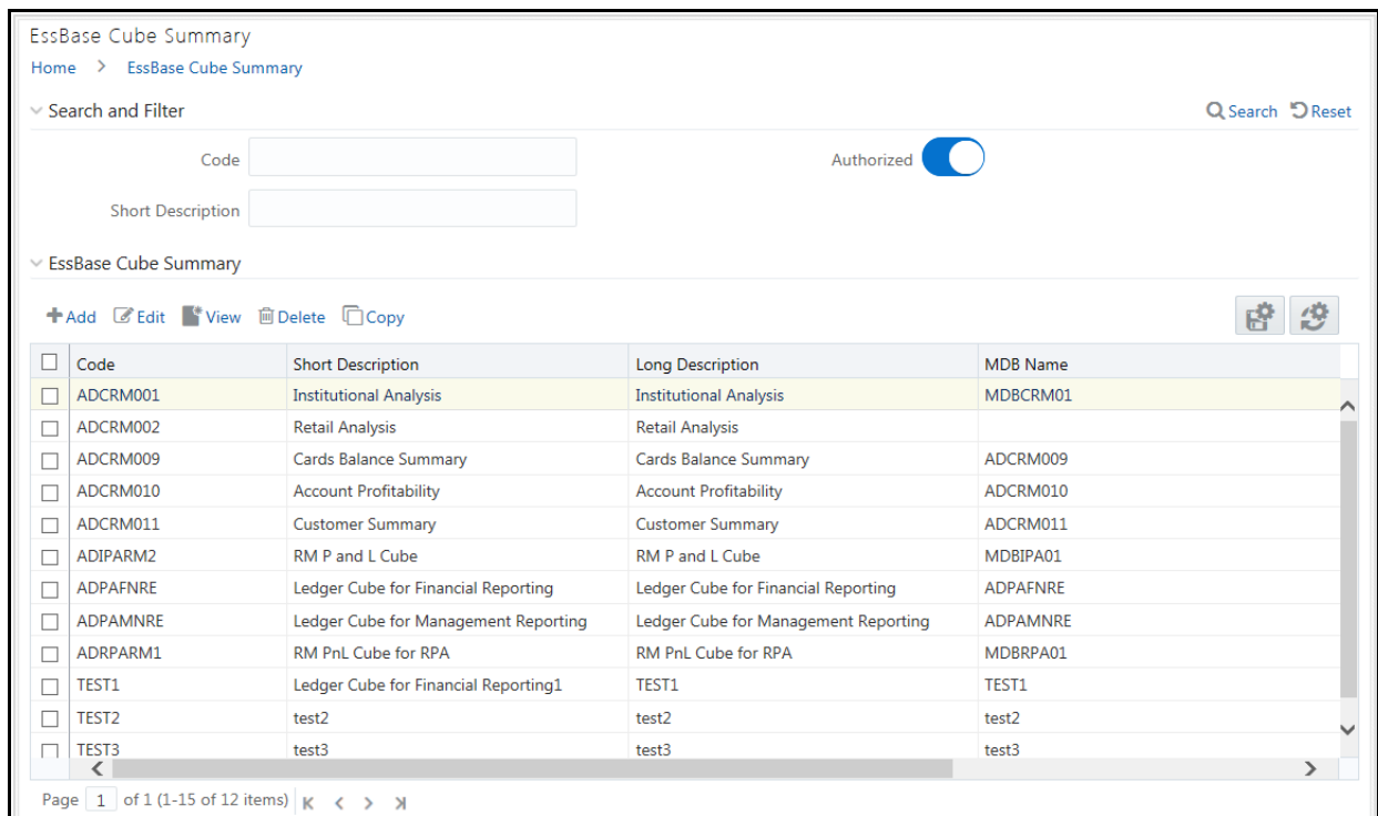
Figure 126: EssBase Cube Summary window
