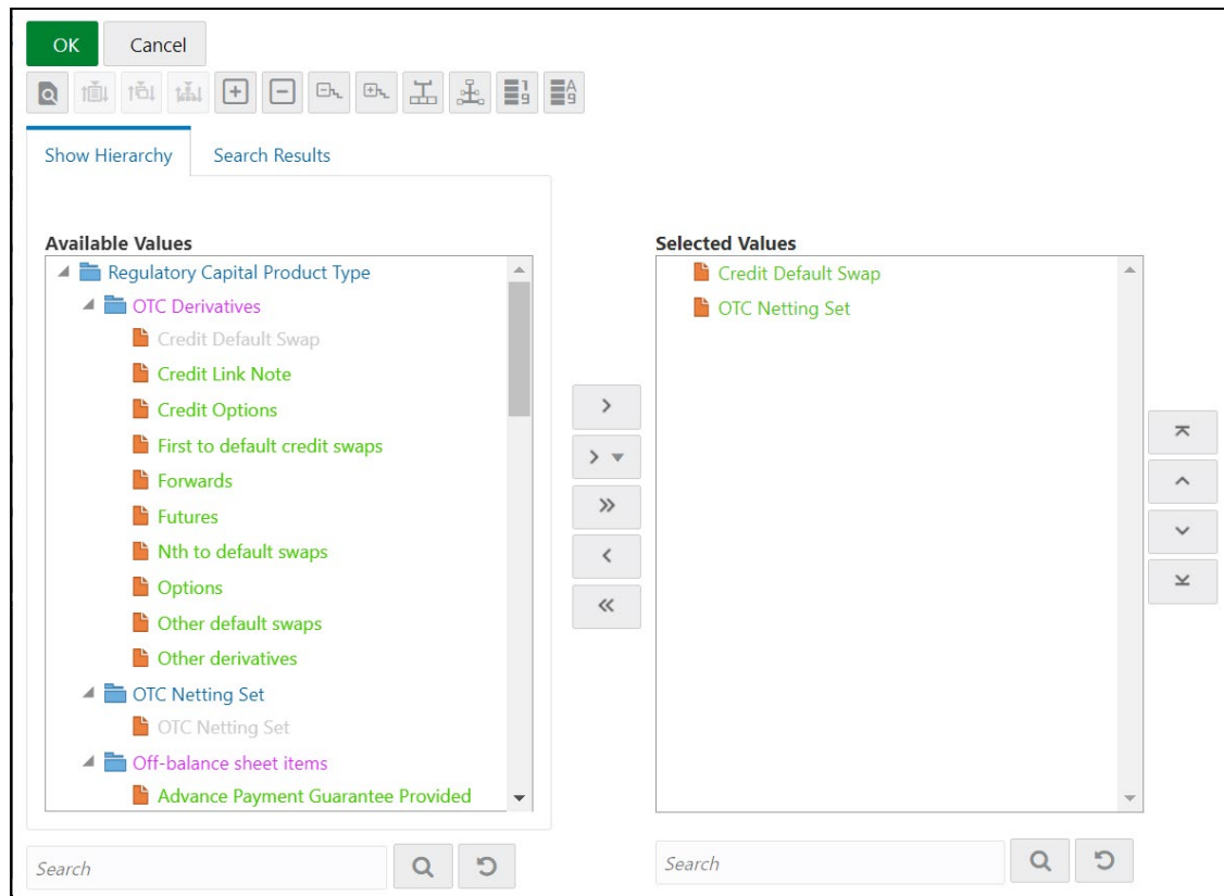
Figure 205: Hierarchy Browser window
