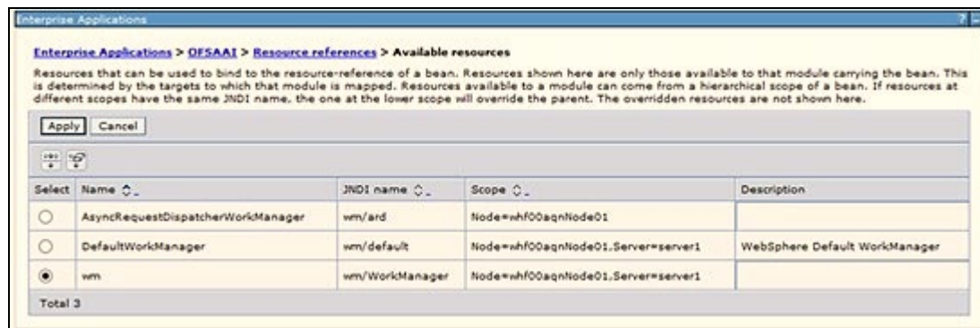
Figure 127: Available Resources
