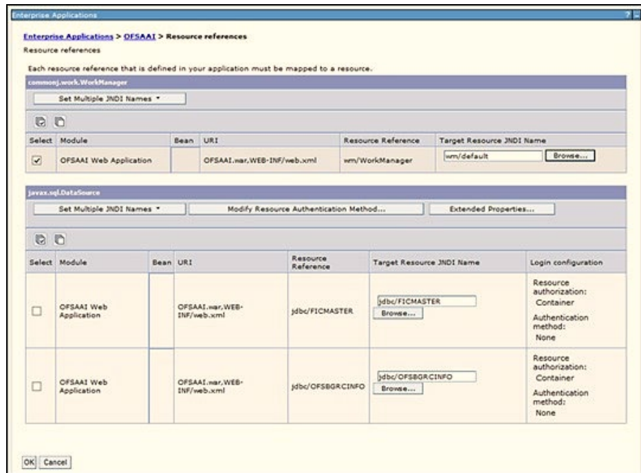
Figure 126: Resource References
