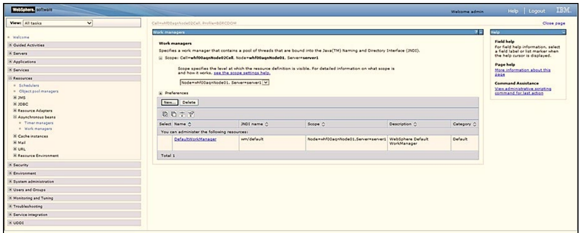
Figure 120: Work Managers
