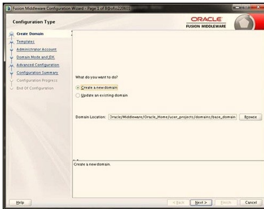
Figure 74: Configuration Type
