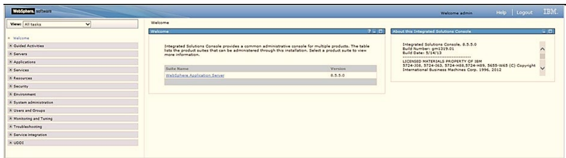
Figure 119: Home page
