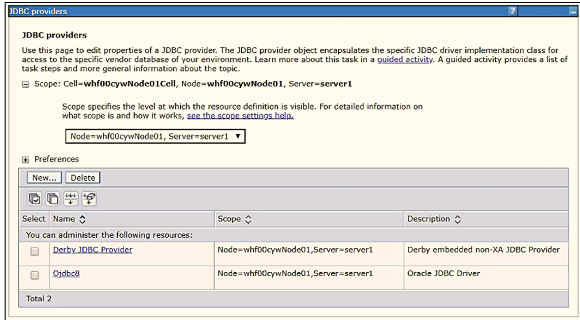
Figure 87: JDBC Providers
