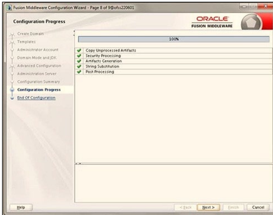
Figure 81: Creating Domain
