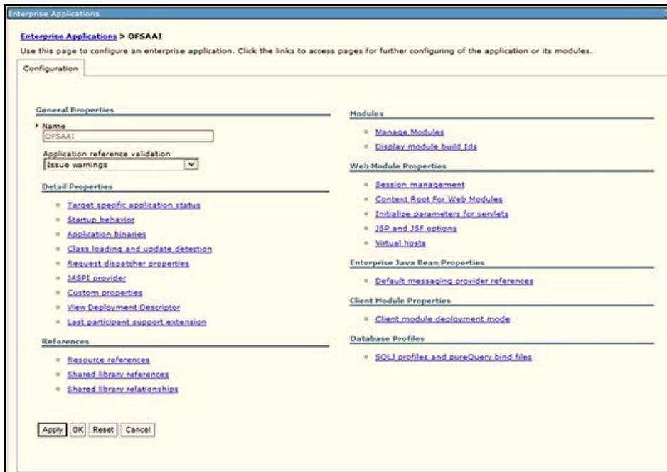
Figure 125: OFSAAI
