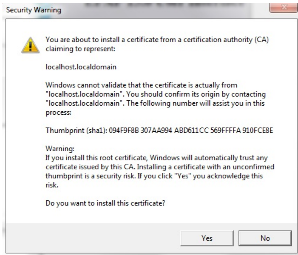
Figure 3-17 Security Warning
