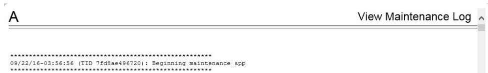
Figure 3-61 Log Viewer
