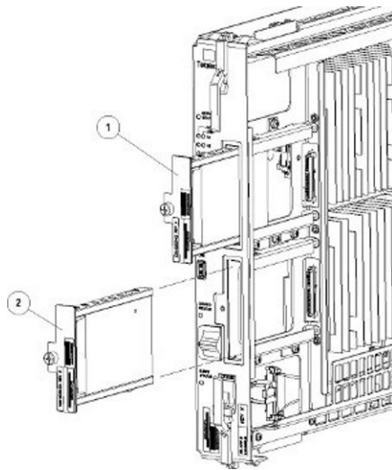
Figure 5-9 Drive Module Removal
