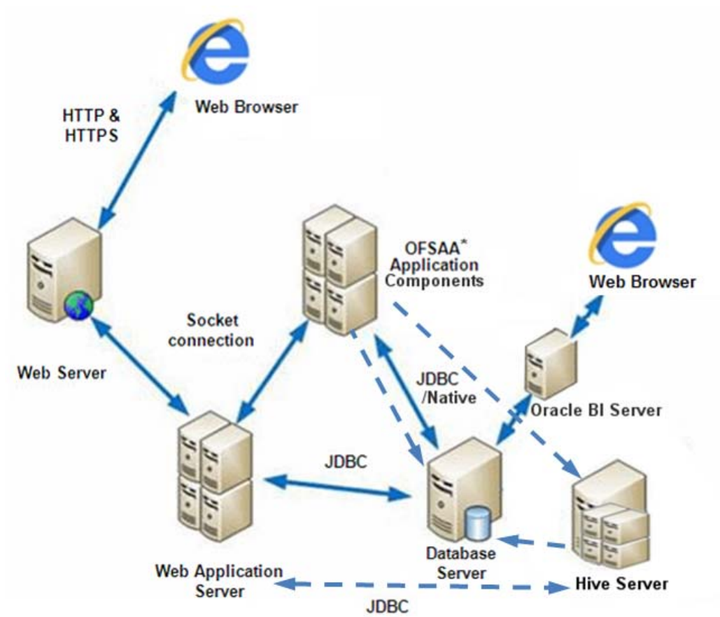
Figure 2-2 Deployment Topology
