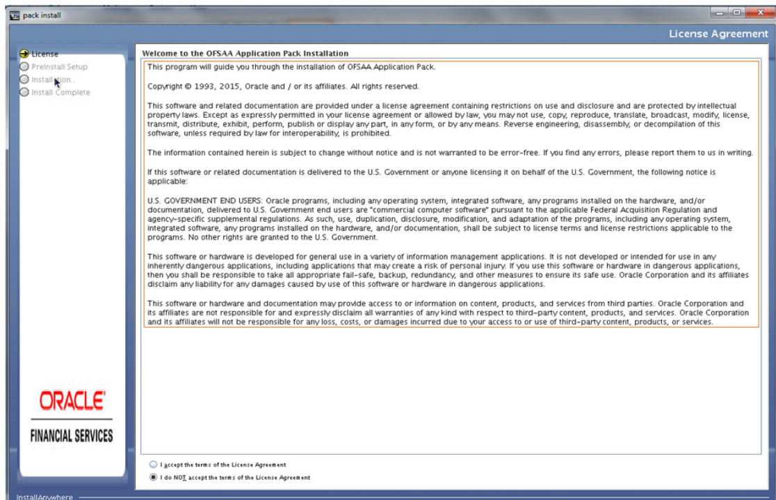
Figure 4–14 License Agreement
