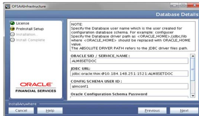
Figure 4–29 Ports Configuration
