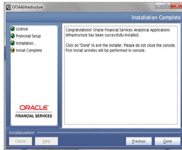
Figure 4-36 Installation Complete
