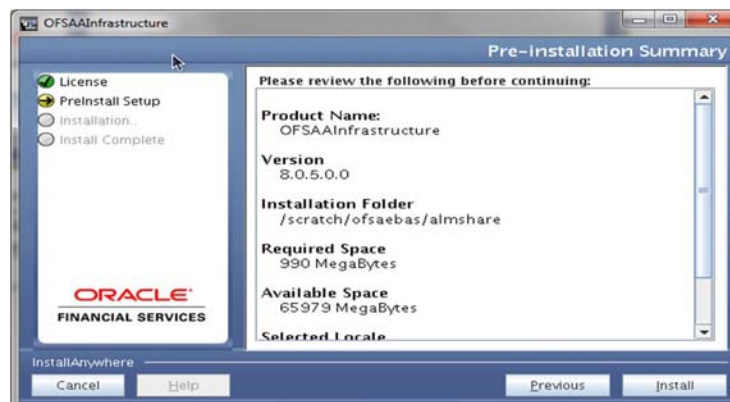
Figure 4-33 Pre-installation Summary
