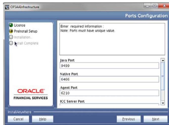
Figure 4–30 Ports Configuration
