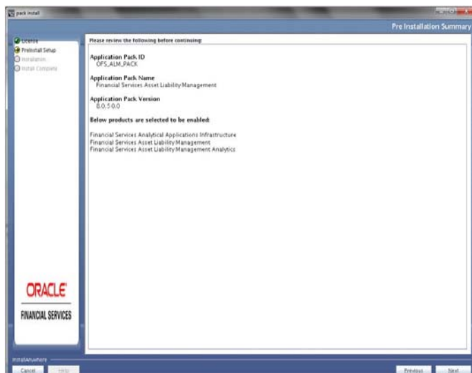
Figure 4–17 Pre-Installation Summary
