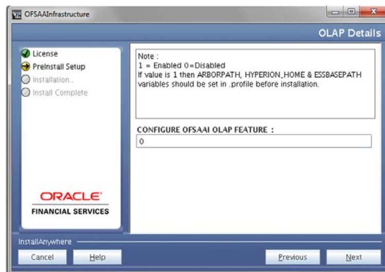
Figure 4–26 OLAP Details
