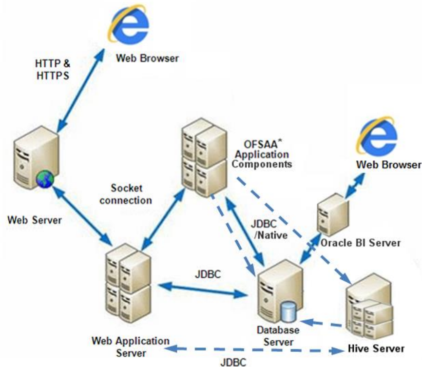
Figure 2-2 Deployment Topology
