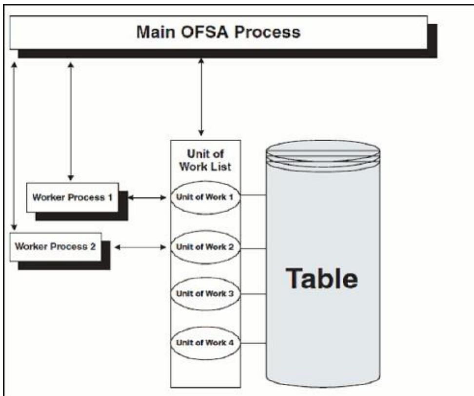
Figure 11: Basic Multiprocessing principles
