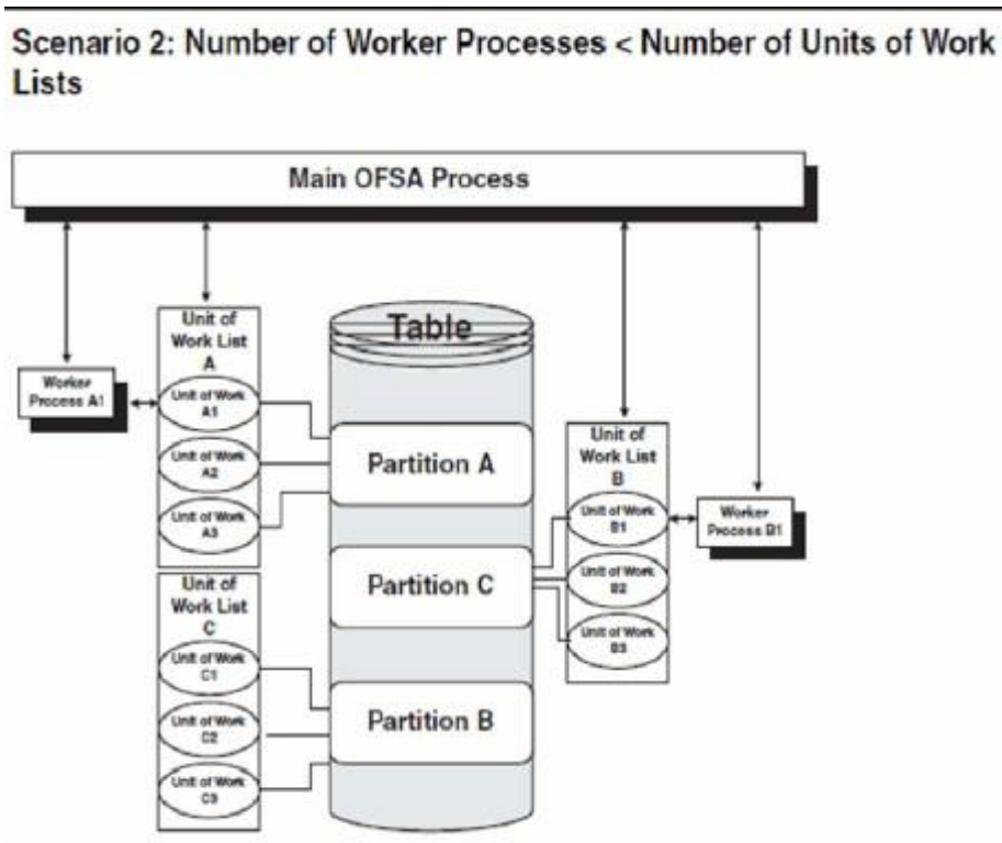
Figure 13: How different units of work are processed at the same time by different worker processes
