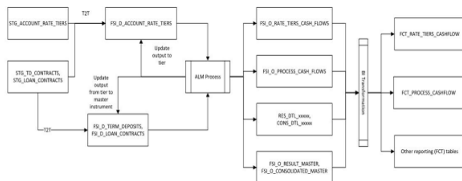
ALM Data Flow
