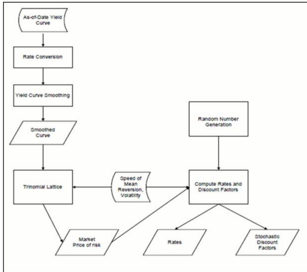
Process flow for Vasicek (or Merton)
