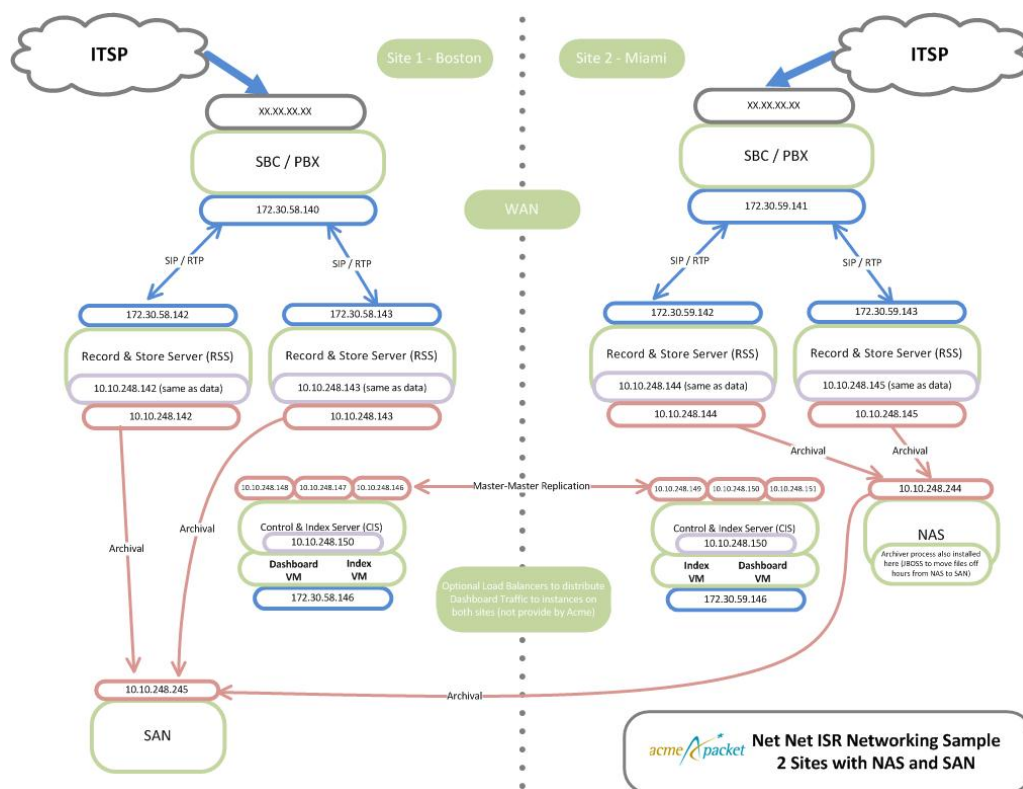
Figure 2-3 Dual Site Redundant ISR/SBC Implementation
