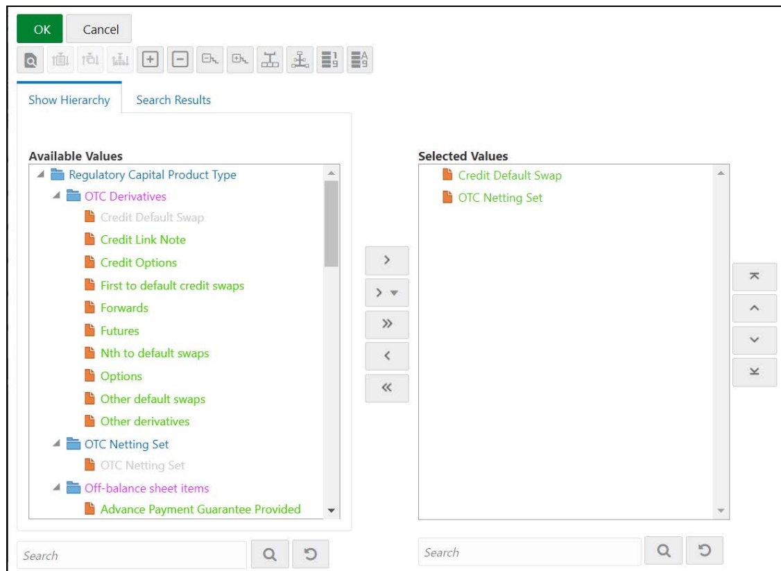
Figure 57: Hieracrchy Selection
